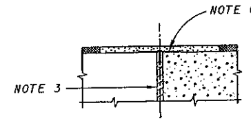
DETAIL E
