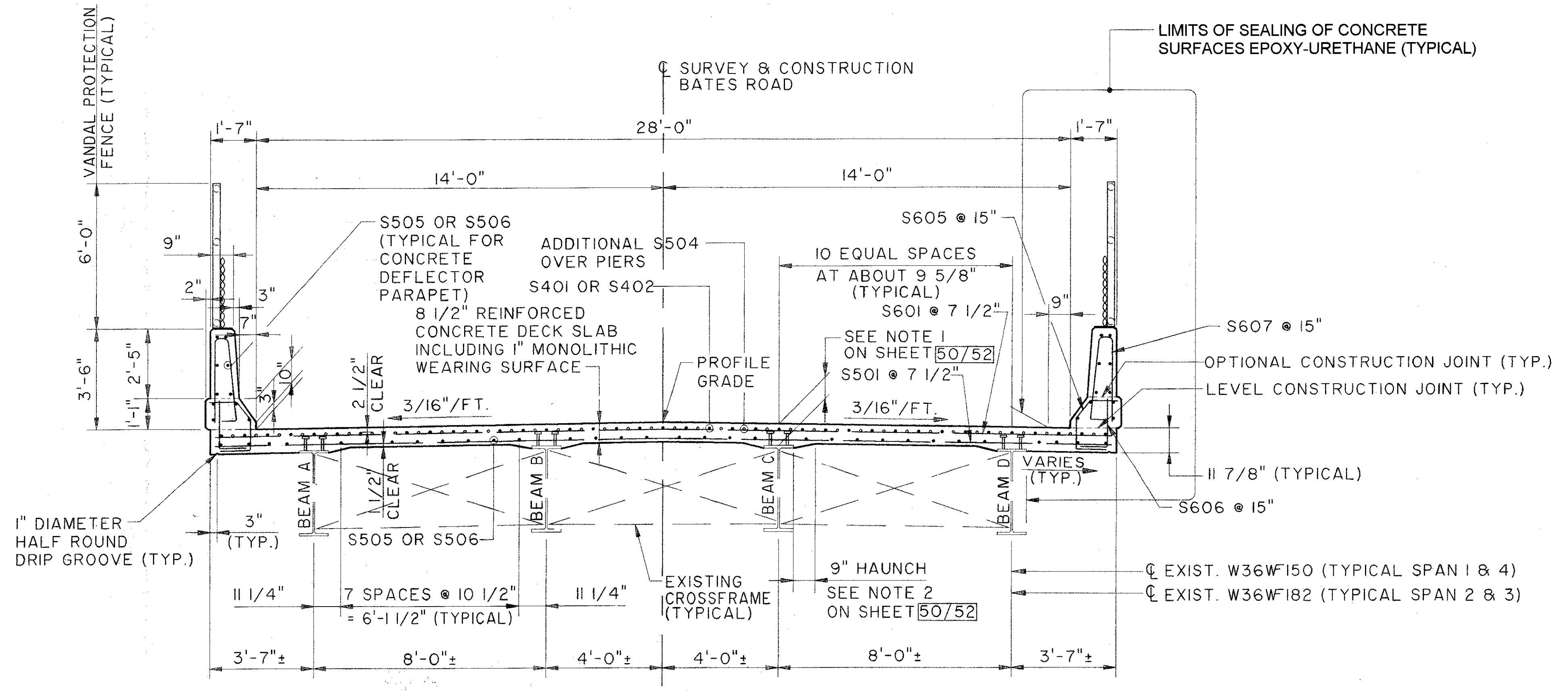
TRANSVERSE DECK SECTION
