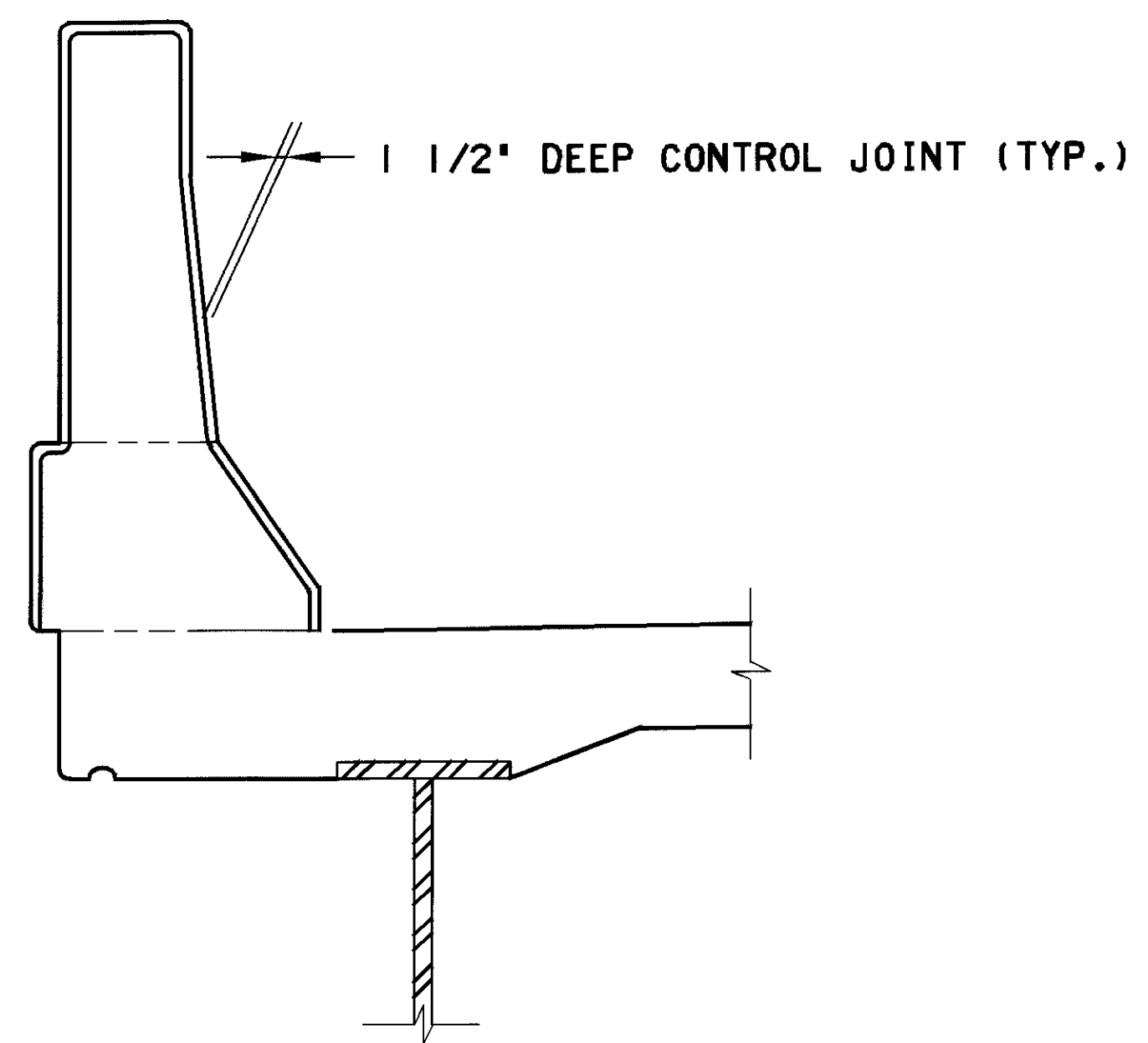
TYPICAL CONTROL JOINT DETAIL
