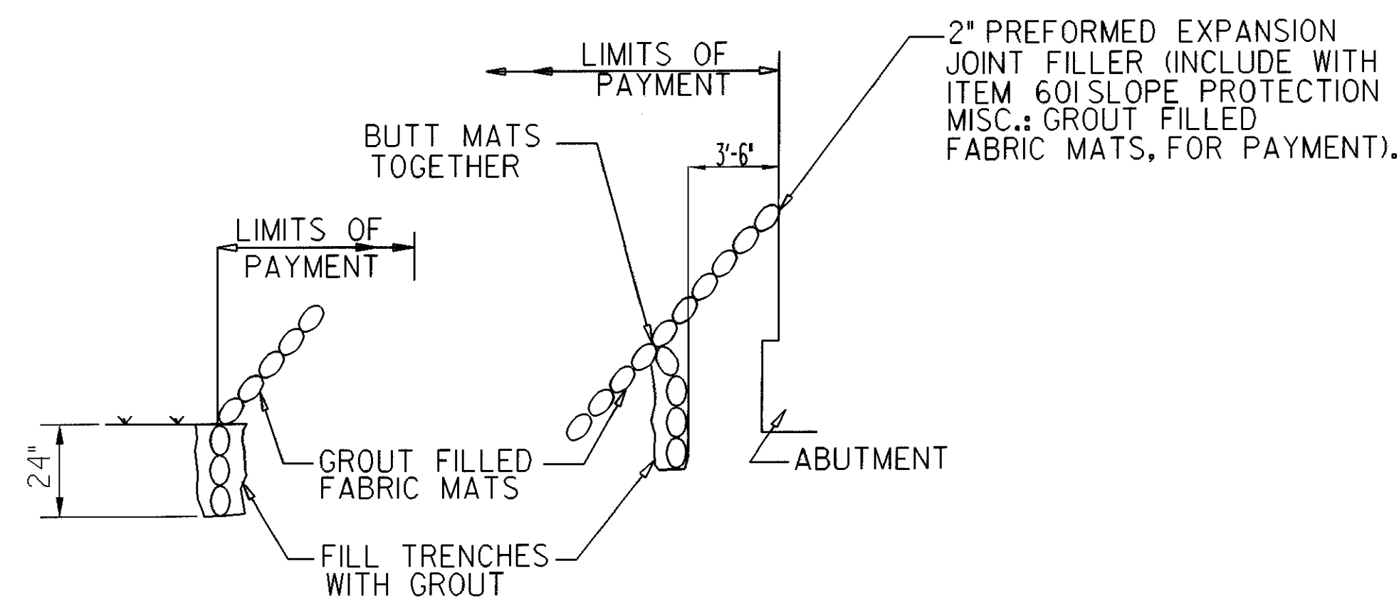
GROUT FILLED FABRIC MAT DETAIL
