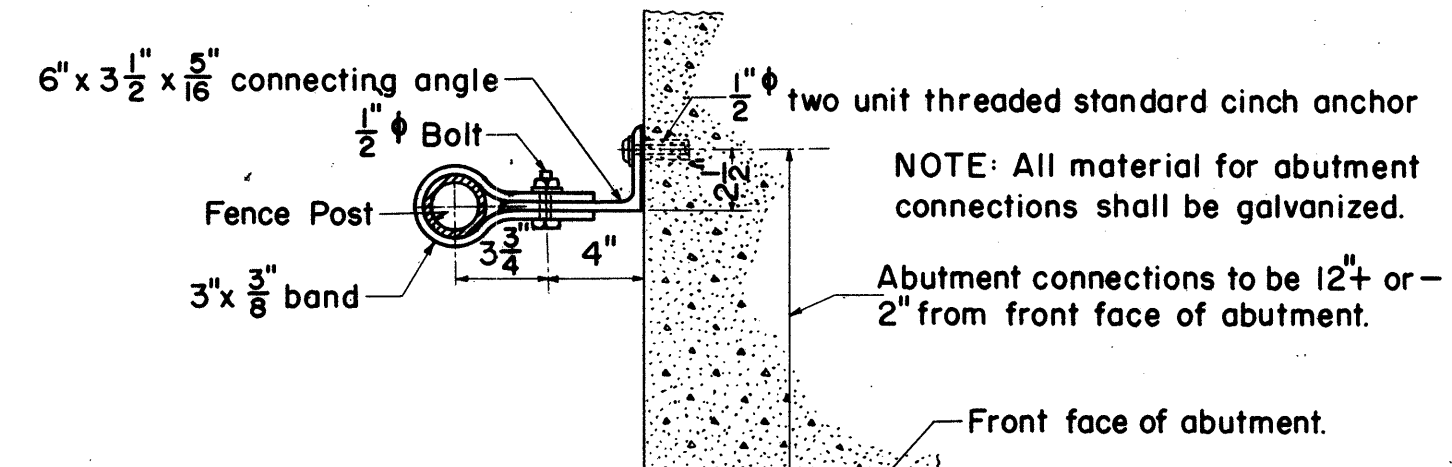
ABUTMENT CONNECTION
