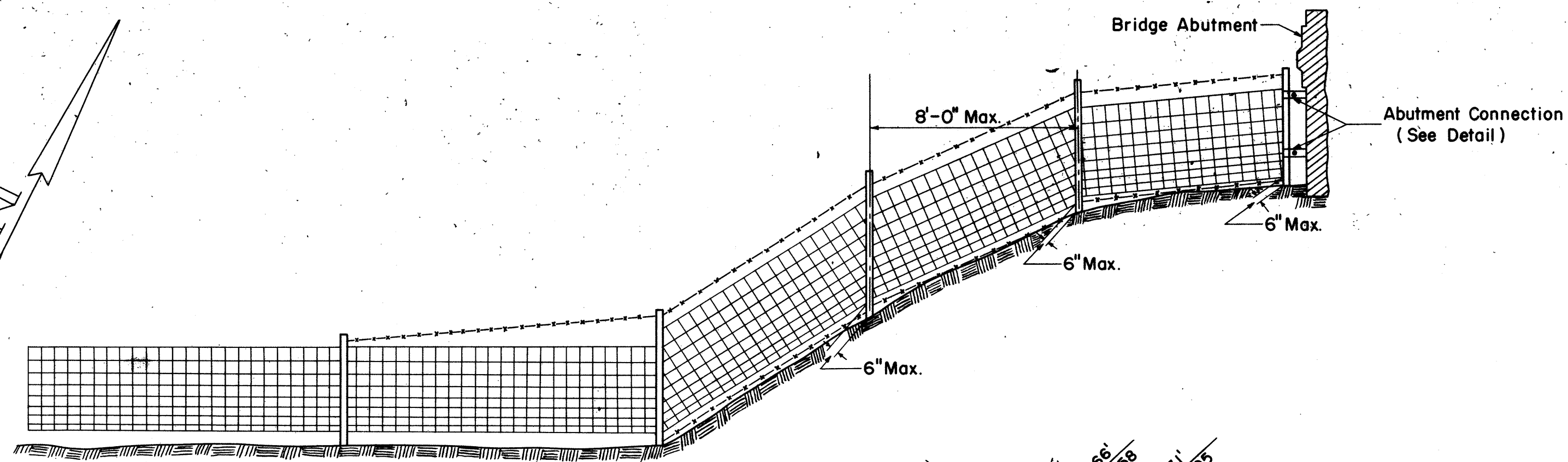
TYPE "A" FENCE SCALE: 1/4" = 1'-0"
