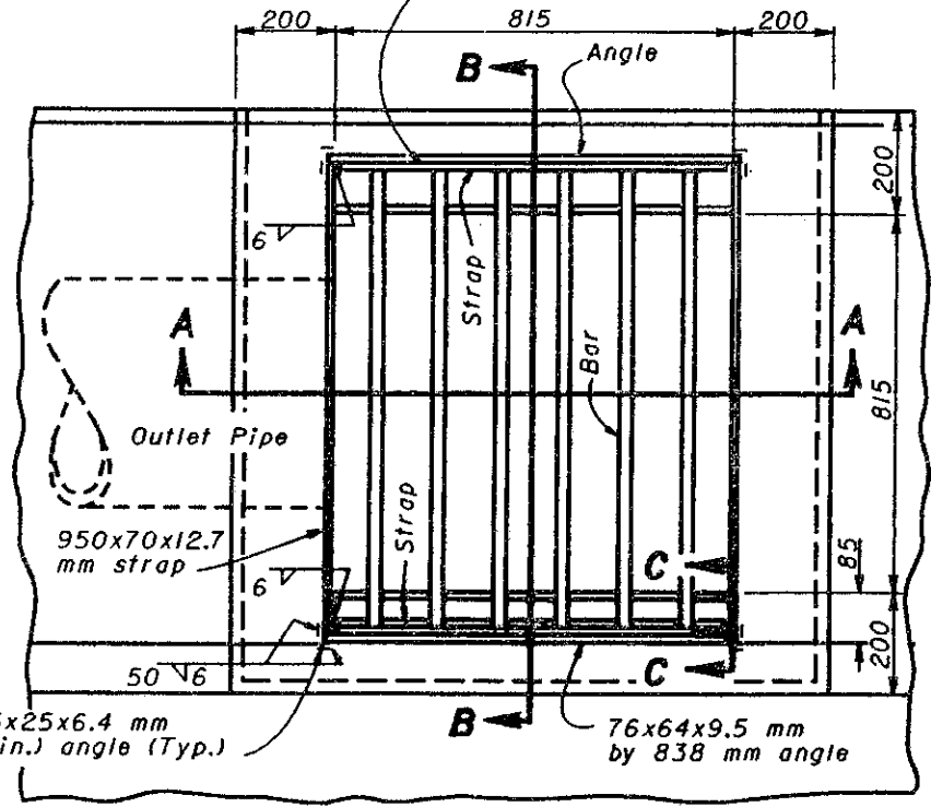
PLAN OF CATCH BASIN
