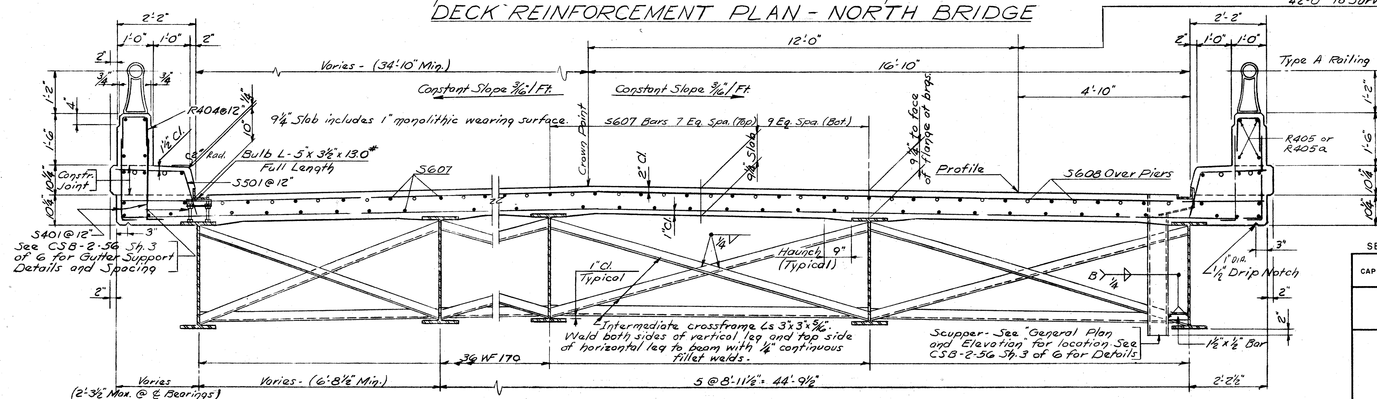
TYPICAL SECTION - NORTH BRIDGE
