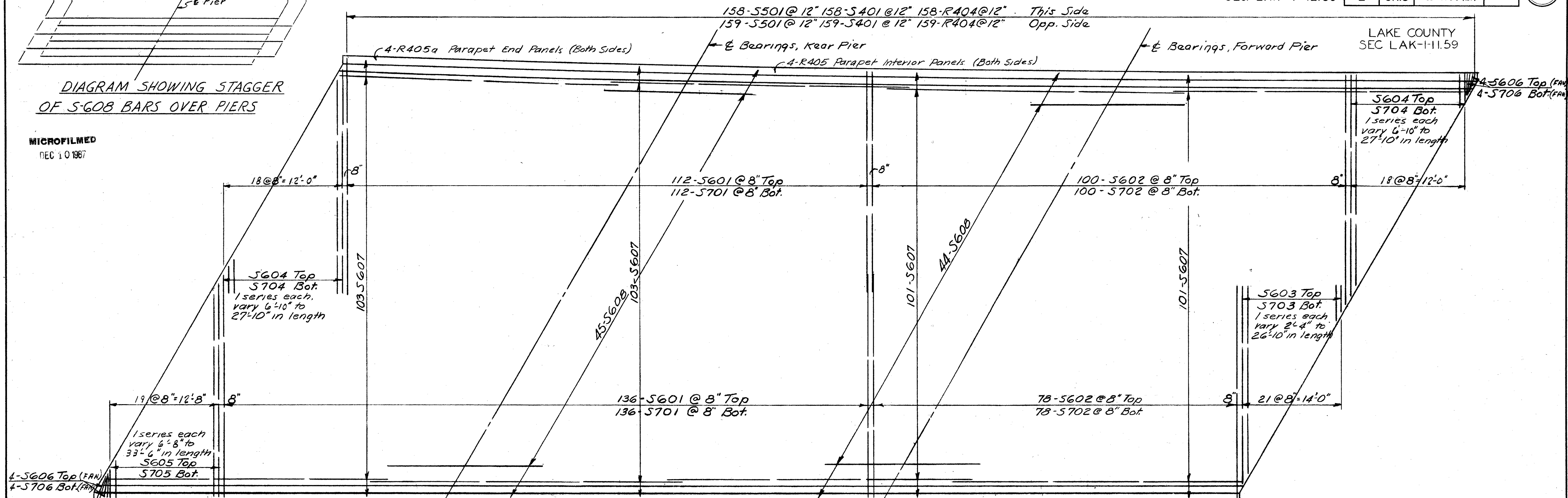
DECK REINFORCEMENT PLAN - NORTH BRIDGE
