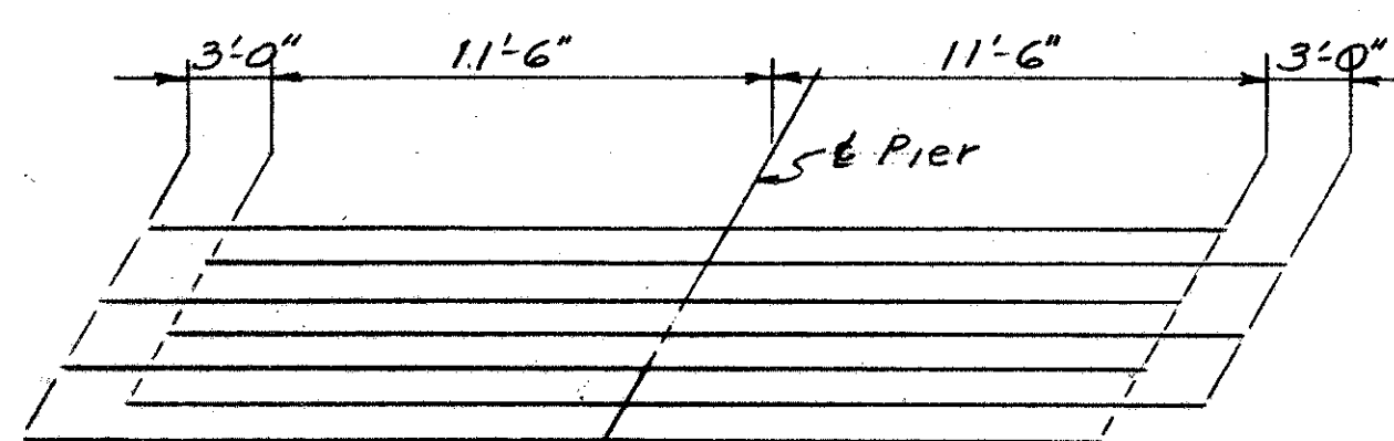
DIAGRAM SHOWING STAGGER OF S-608 BARS OVER PIERS
