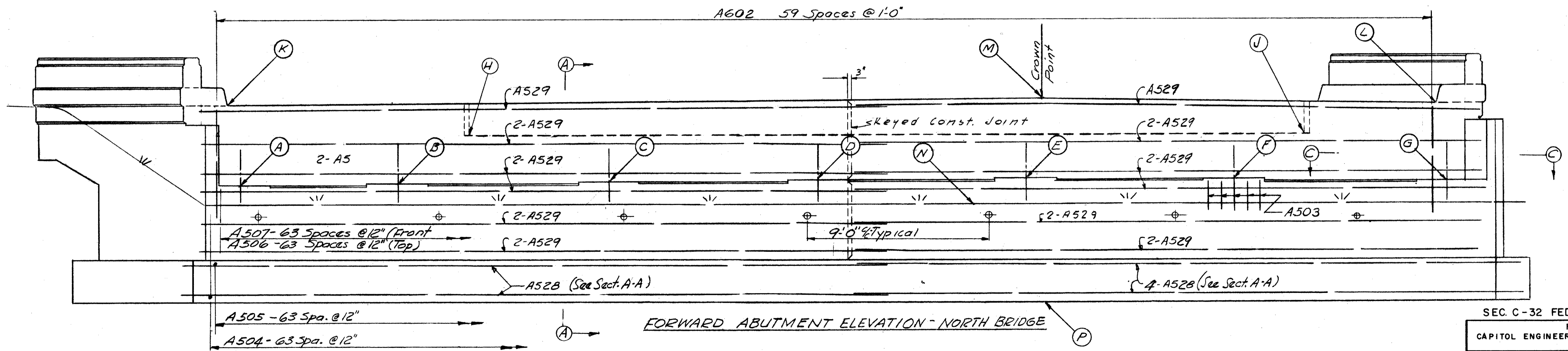
FORWARD ABUTMENT PLAN - NORTH BRIDGE
