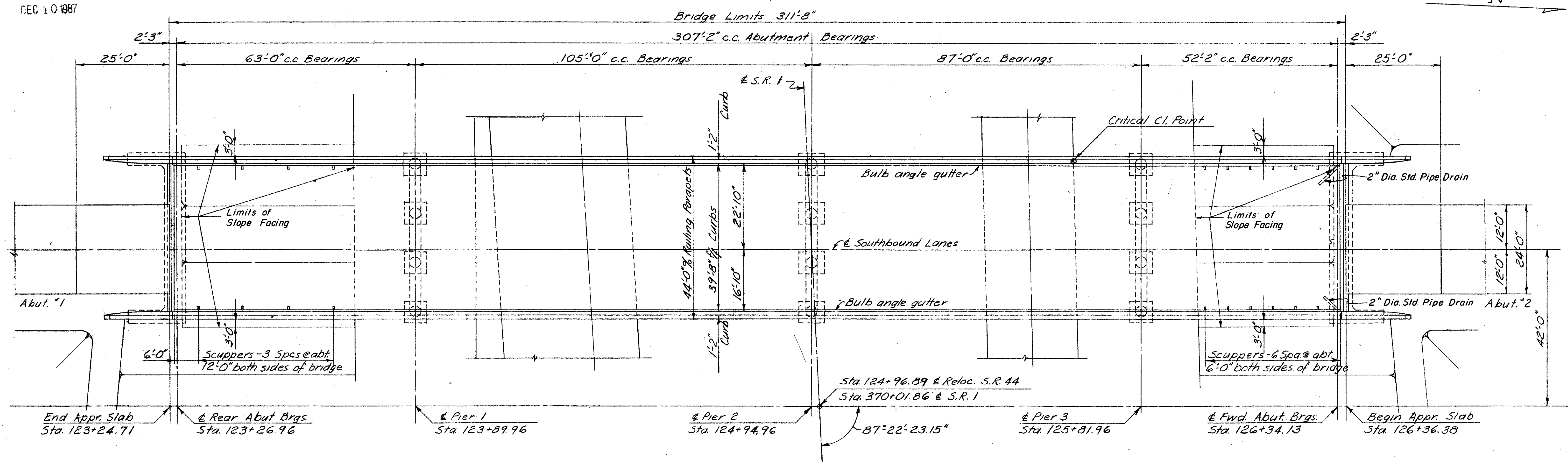
GENERAL PLAN
