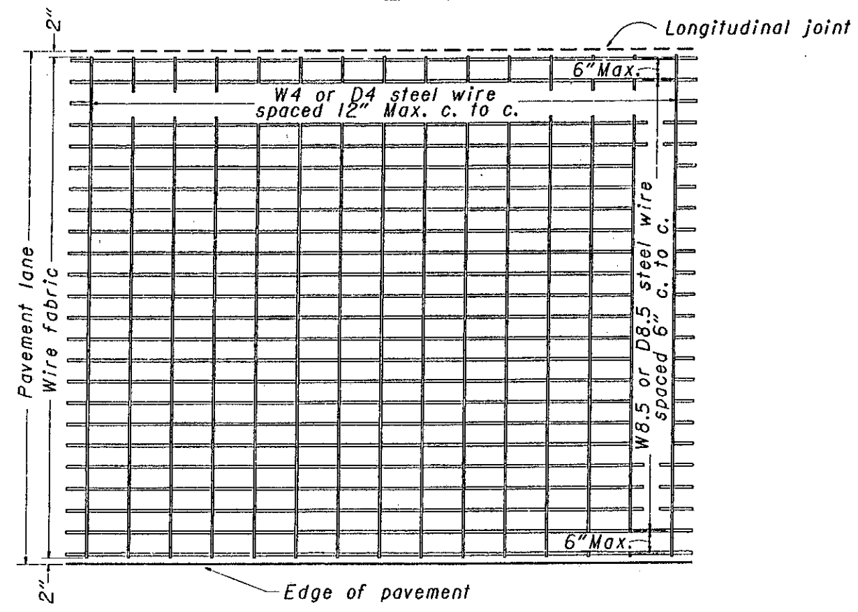
WIRE FABRIC DETAIL
