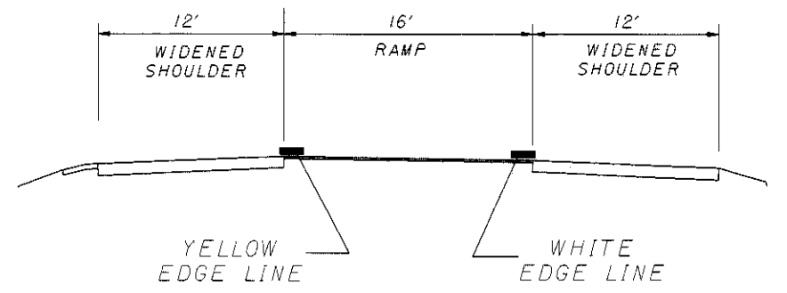
PAVEMENT MARKING TYPICAL LOOKING IN THE DIRECTION OF TRAFFIC
