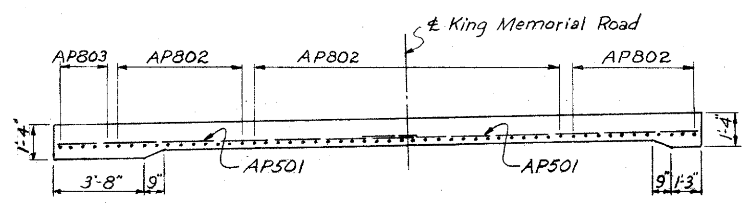
SECTION B-B
