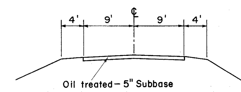
TYPICAL SECTION EXISTING HERMITAGE RD.
