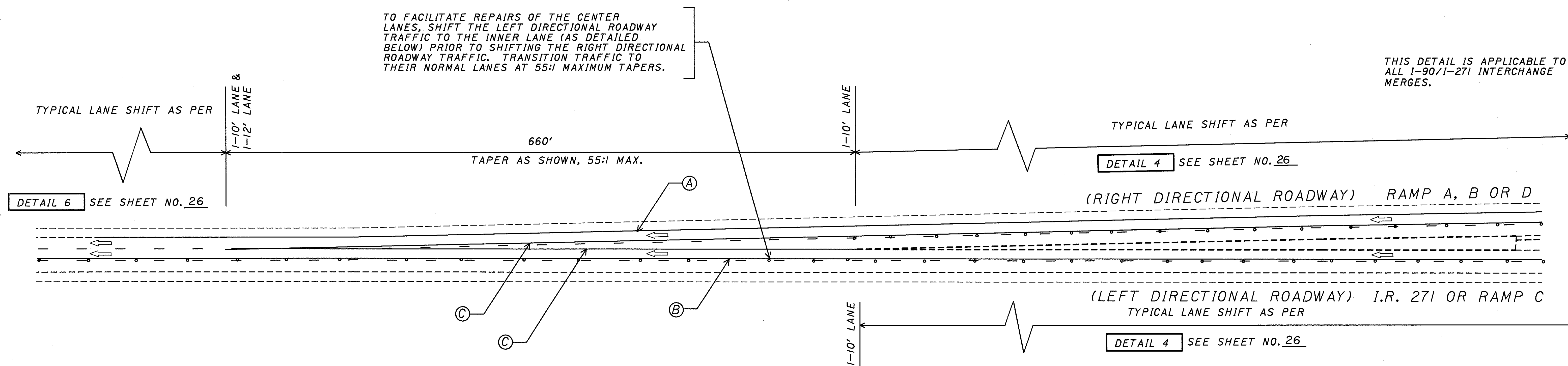
I.R. 271/I.R. 90 MERGE PHASE I - LEFT LANE CLOSED
