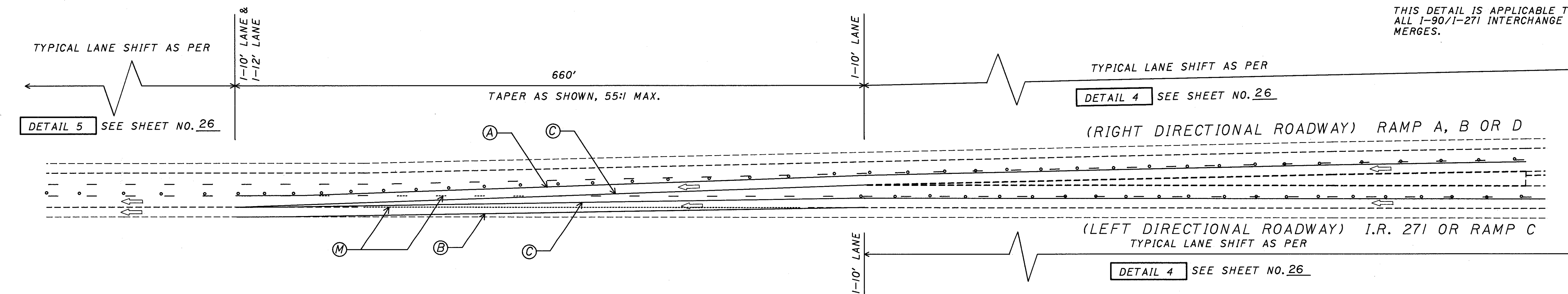
I.R. 271/I.R. 90 MERGE PHASE II - RIGHT LANE CLOSED
