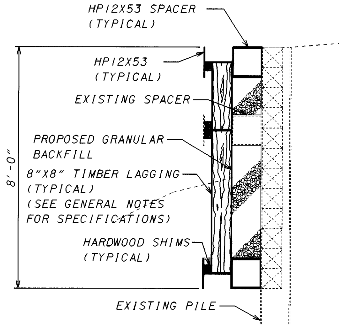
SECTION C-C
