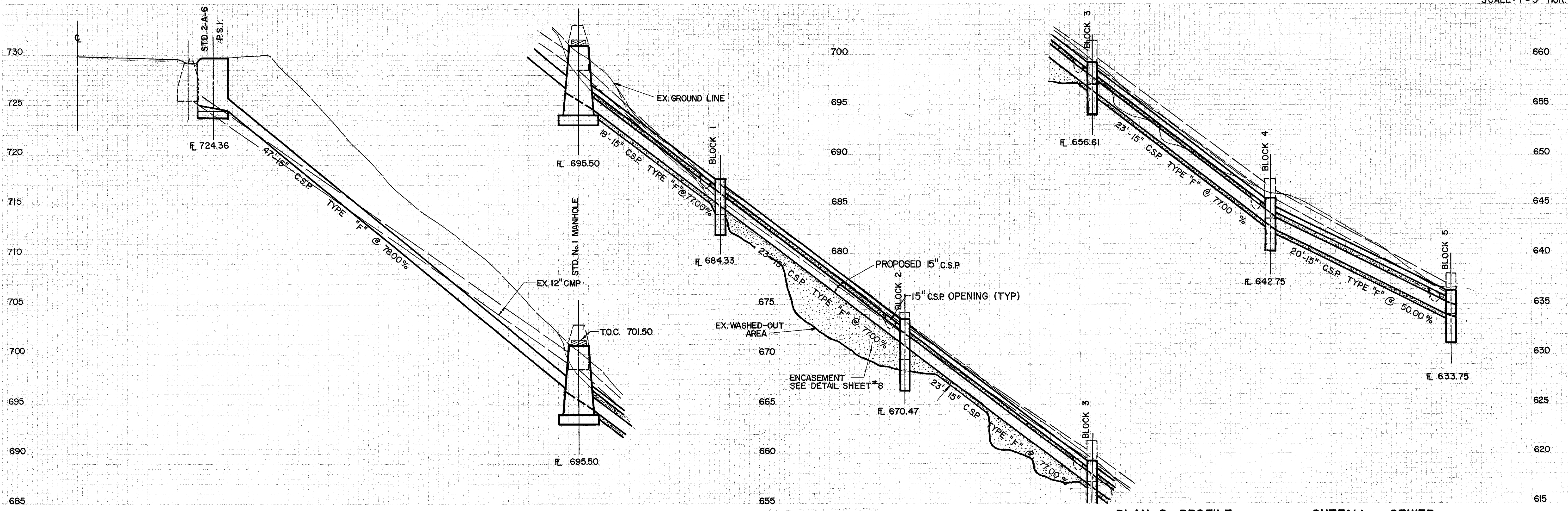
PLAN & PROFILE OUTFALL SEWER
