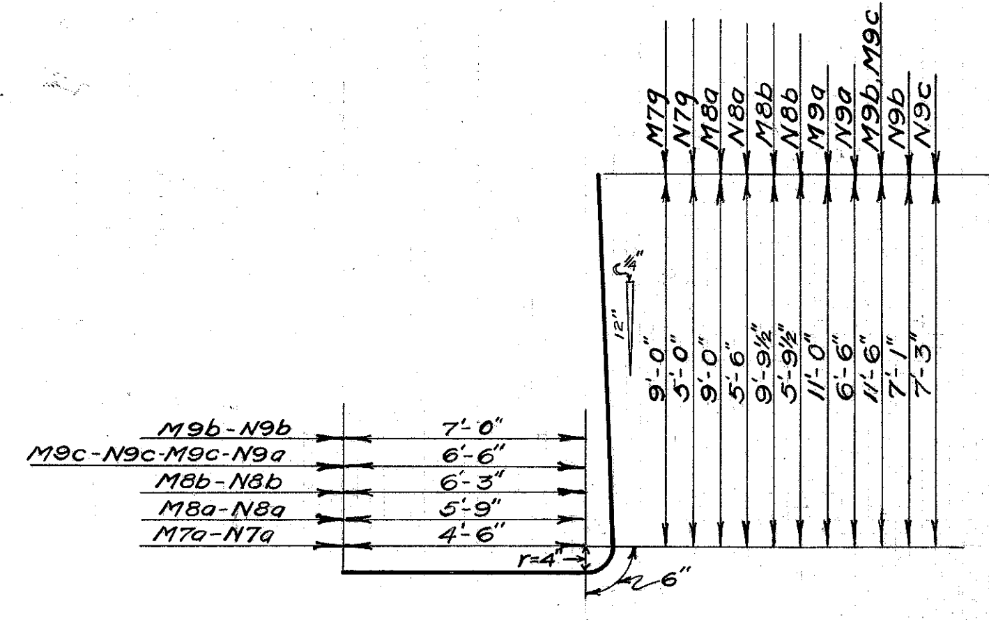
BAR BENDING DIAGRAMS
