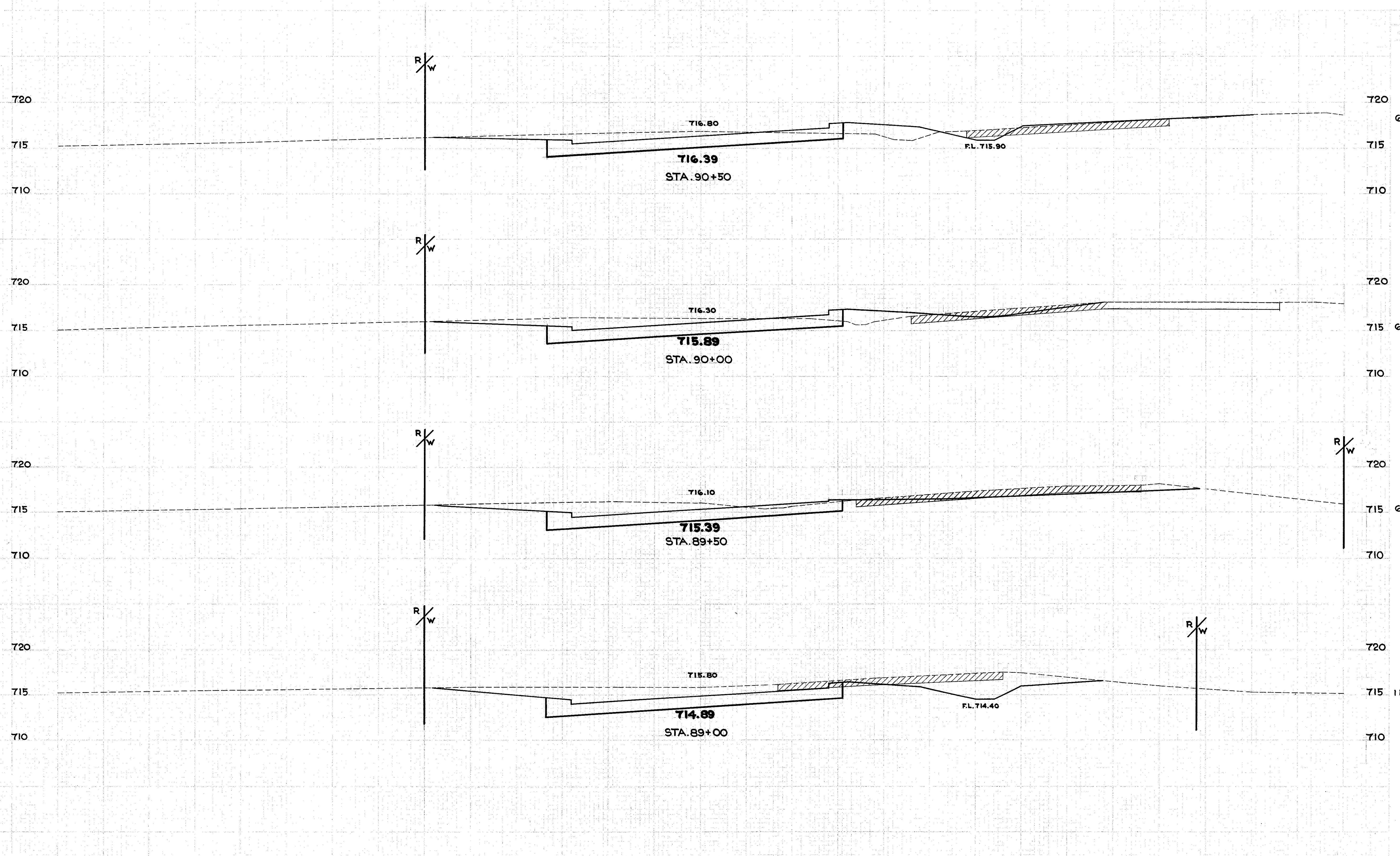
CROSS SECTIONS ... S.R. 84... STA.89+00 to STA.90+50
