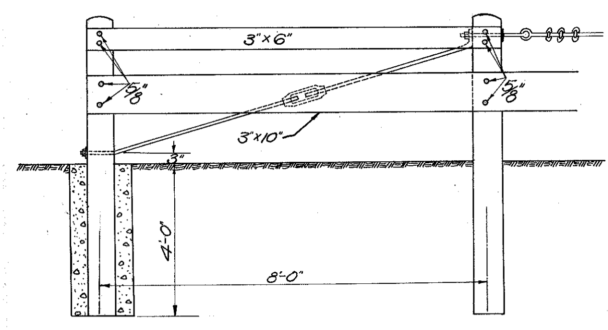
Detail of Anchor to be used for Guard Rail Abutting Bridge
