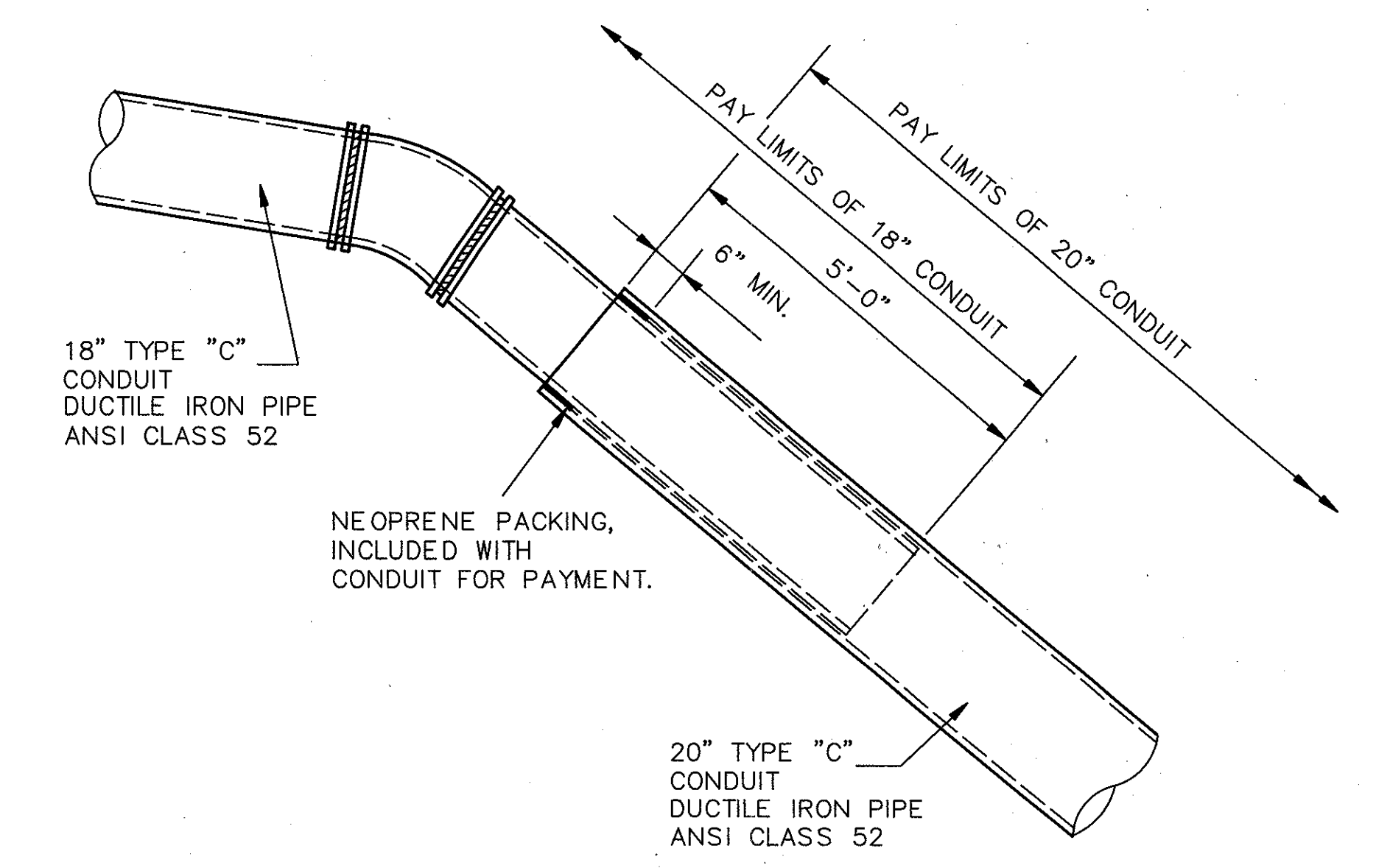
PIPE CONNECTION DETAIL NO SCALE
