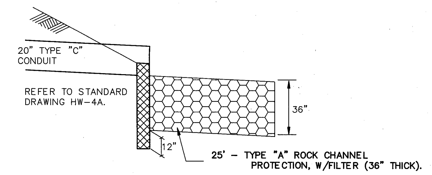
HW-4A, AS PER PLAN DETAIL NO SCALE
