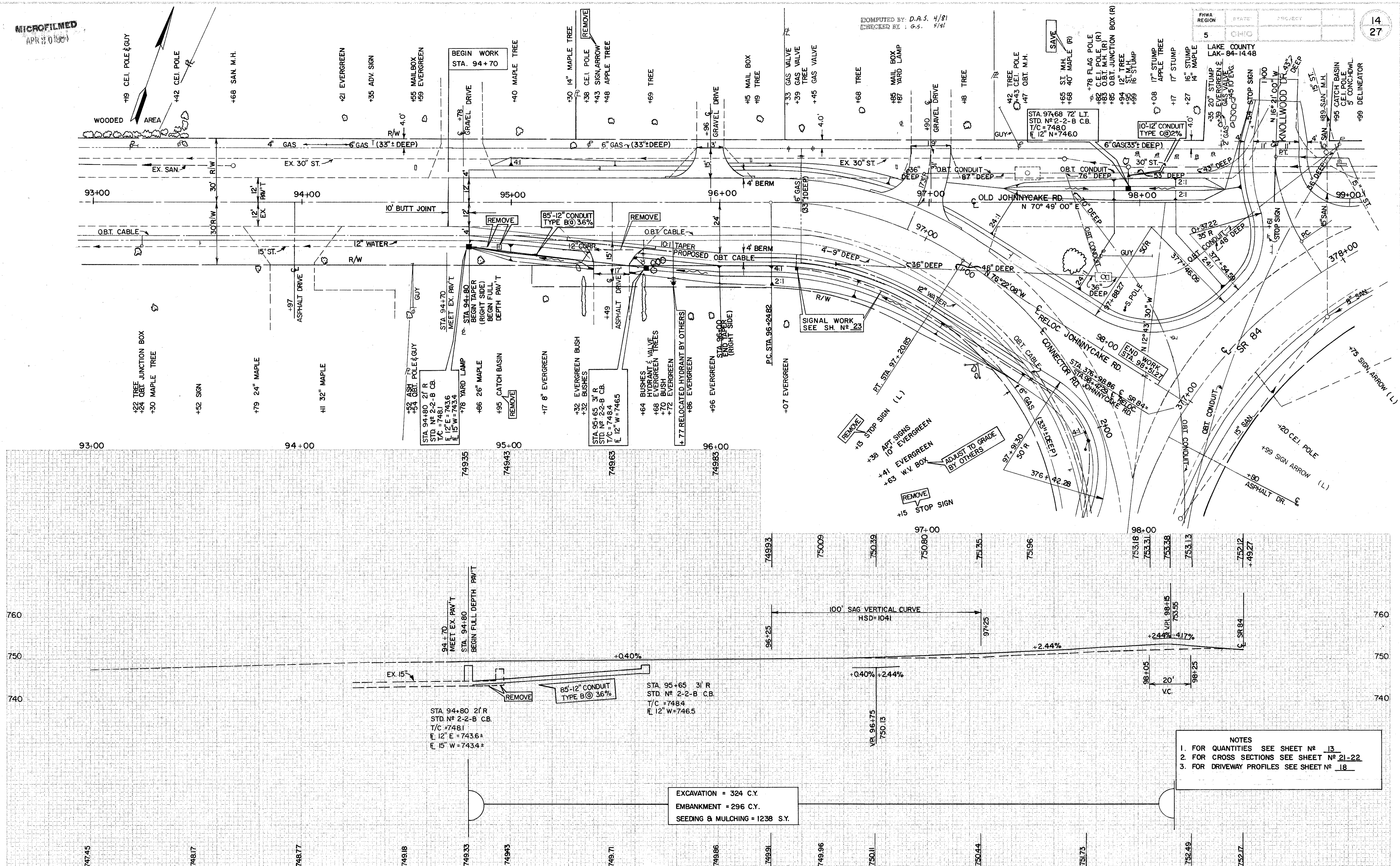
PLAN & PROFILE SHEET RELOCATED JOHNNYCAKE RD. STA. 94+80 TO STA. 98+49.27
