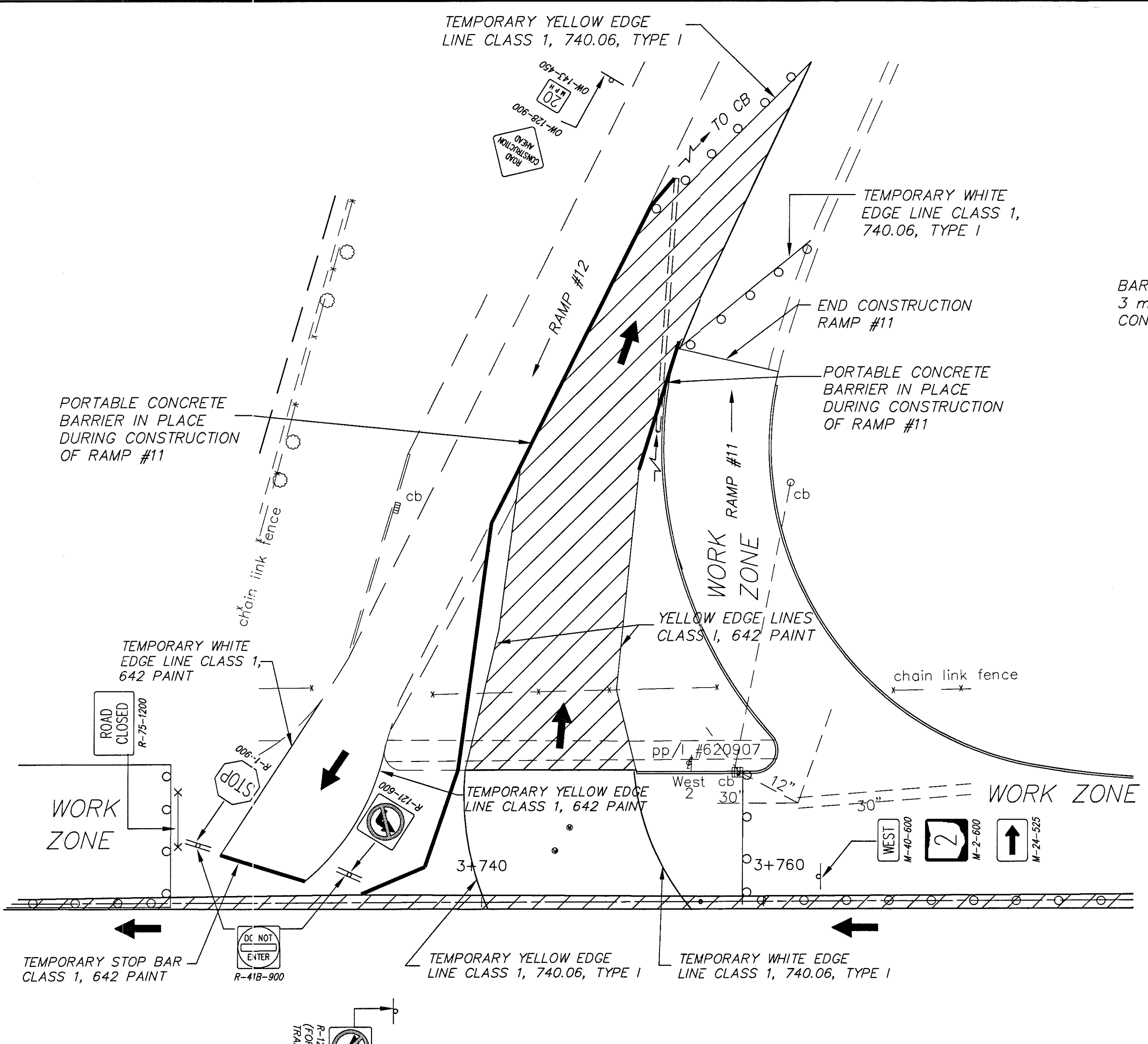
TEMPORARY RAMP DETAIL RAMP #11 CLOSED POSTED SPEED FOR RAMPS (20 MPH)
