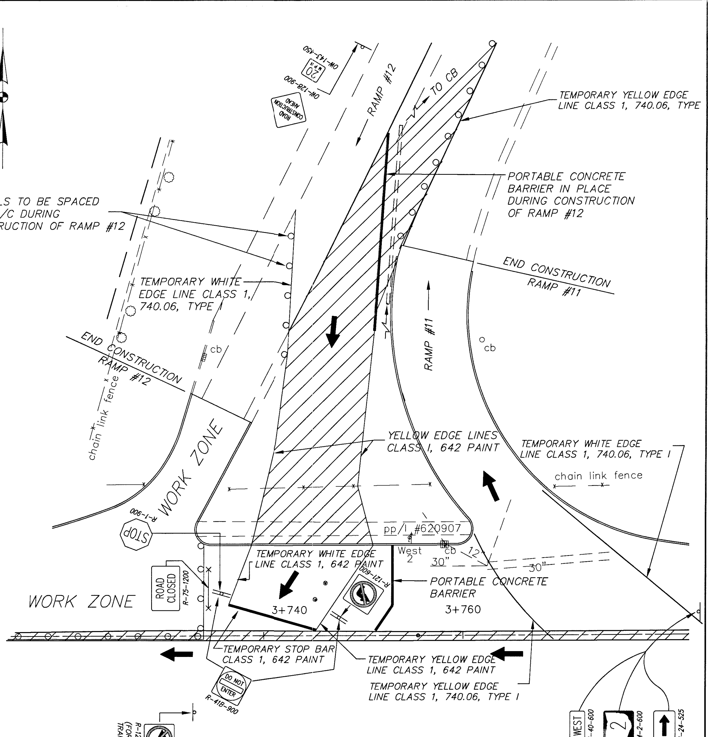
TEMPORARY RAMP DETAIL RAMP #12 CLOSED POSTED SPEED FOR RAMPS (20 MPH)
