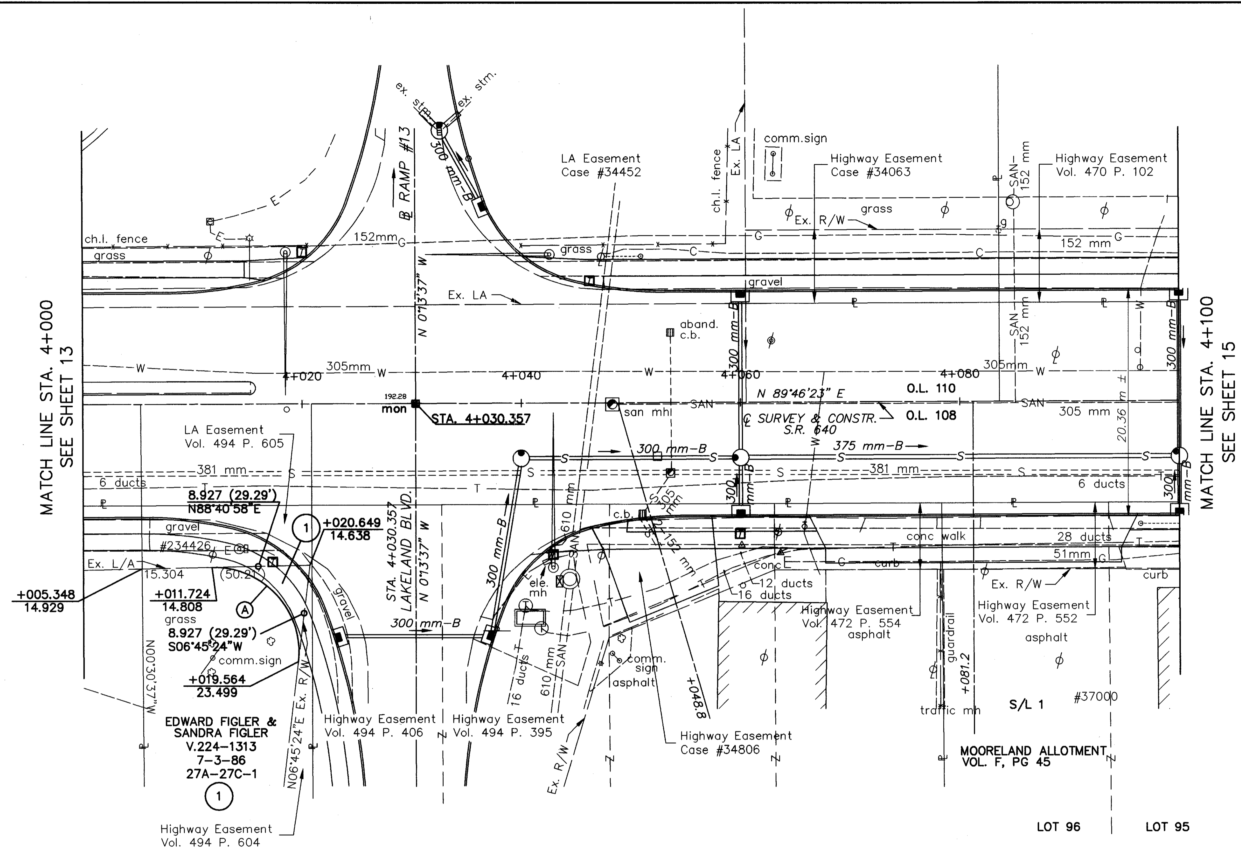
RIGHT OF WAY CURVE DATA
