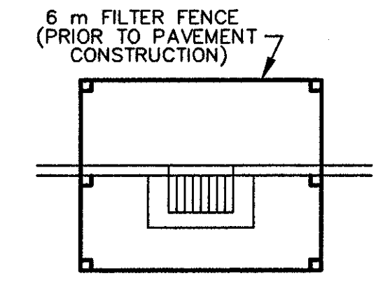
CATCH BASIN BOXOUT W/FILTER FABRIC FENCE AS PER STANDARD DRAWING DM 4.3M NTS
