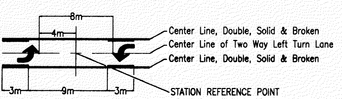
LAYOUT DETAIL FOR TWO WAY LEFT TURN LANES
