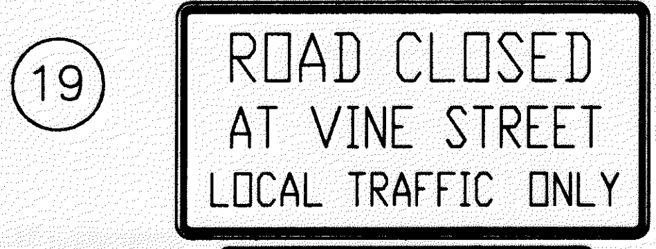
19 R-76A 1524mmX762mm(60"X30") & OC-14R 1219mmX610mm(48"X24") WITH TYPE III BARRICADE
