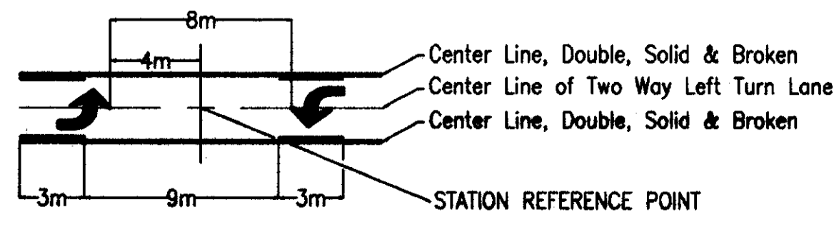
LAYOUT DETAIL FOR TWO WAY LEFT TURN LANES
