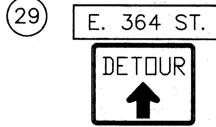
29 STREET SIGN & 762mmX610mm(30"X24") OC-29
