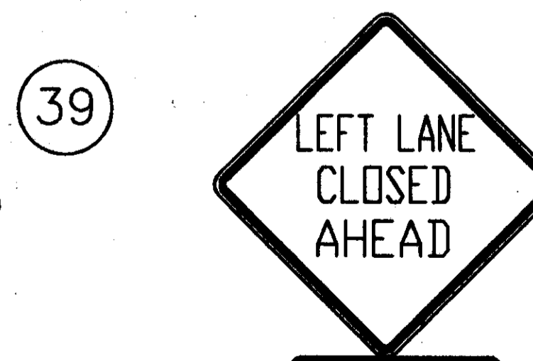
39 OW-123-36 & OW-145B 610mmX457mm(24"X18") (61 METERS PRIOR TO WORK ZONE)
