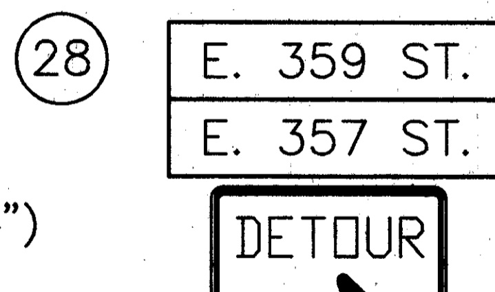
28 2 STREET SIGNS & 762mmX610mm(30"X24") OC-29R
