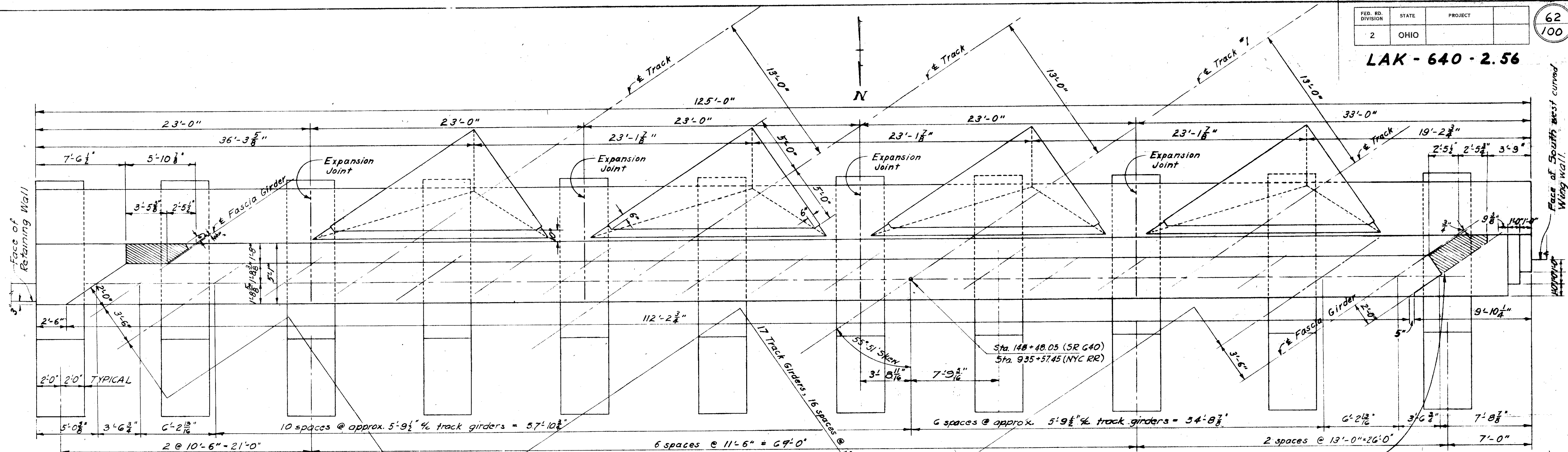
ABUTMENT PLAN
