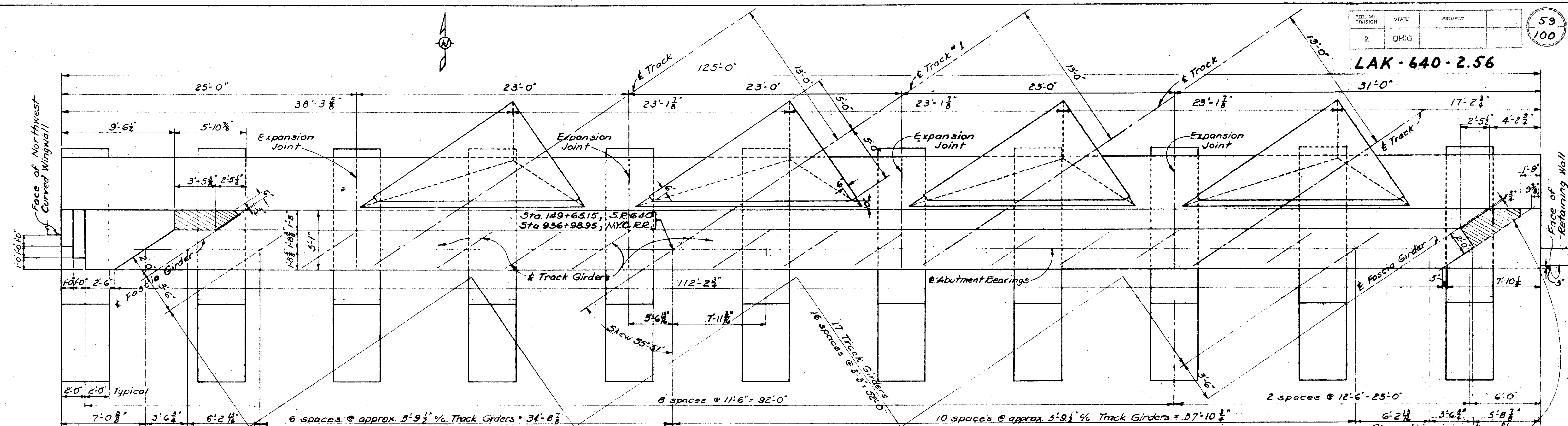
ABUTMENT PLAN
