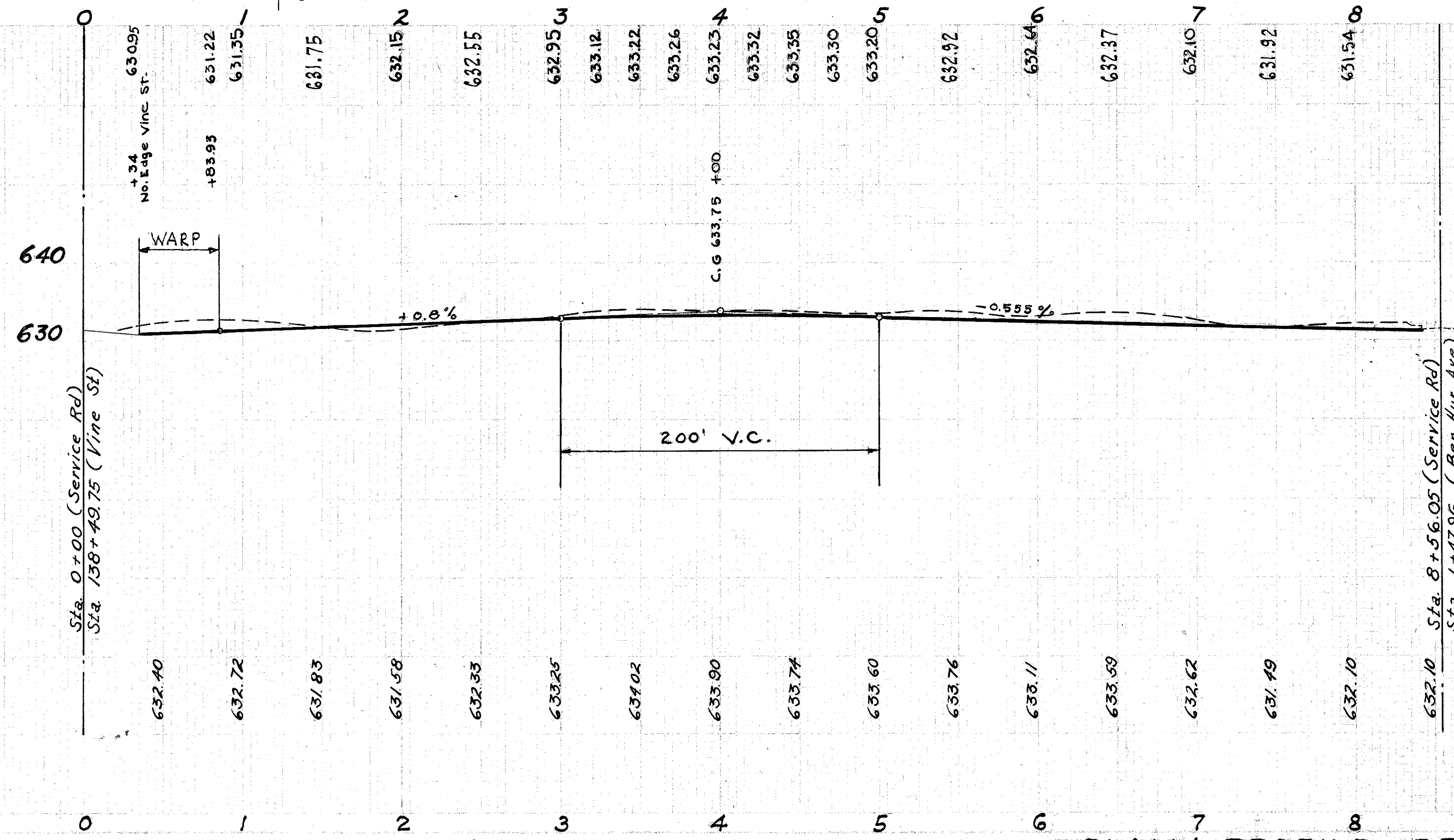
PLAN & PROFILE ~ BEN-HUR SERVICE RD. STA 0+00 TO 8+56.05
