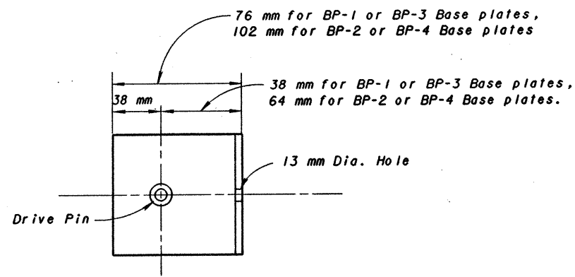
VIEW B-B SHOWING FENCE CLOSURE PLATE PLAN
