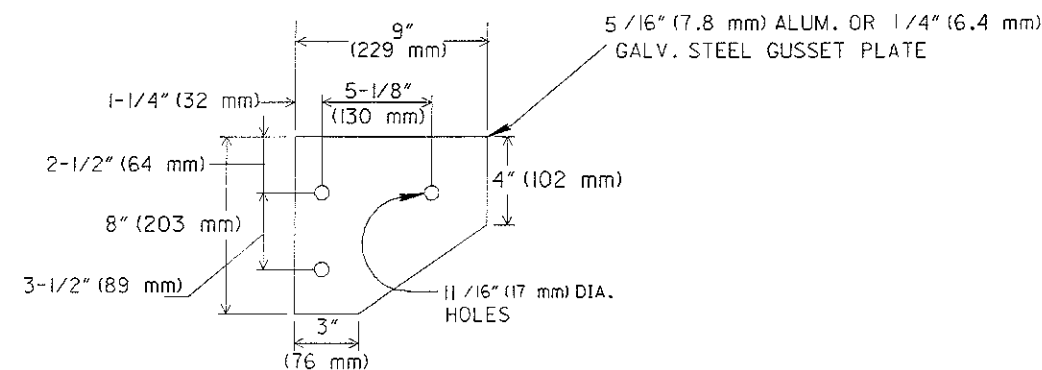
GUSSET PLATE
