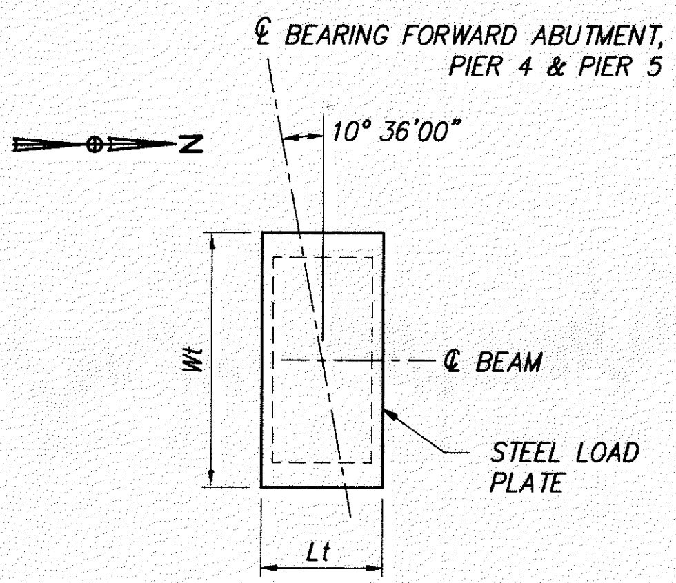
BEARING ORIENTATION PLAN
