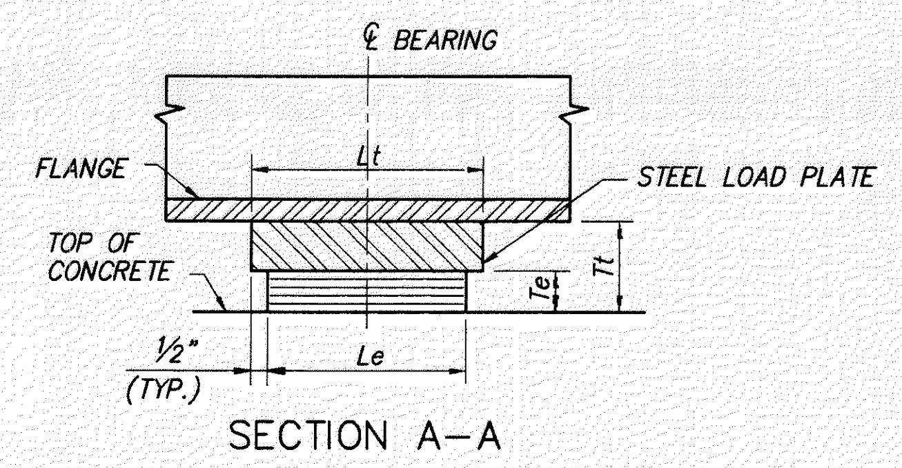
LAMINATED ELASTOMERIC EXPANSION BEARING AT REAR ABUTMENT
