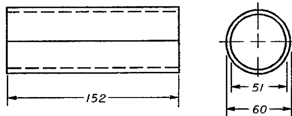
POST SLEEVE
