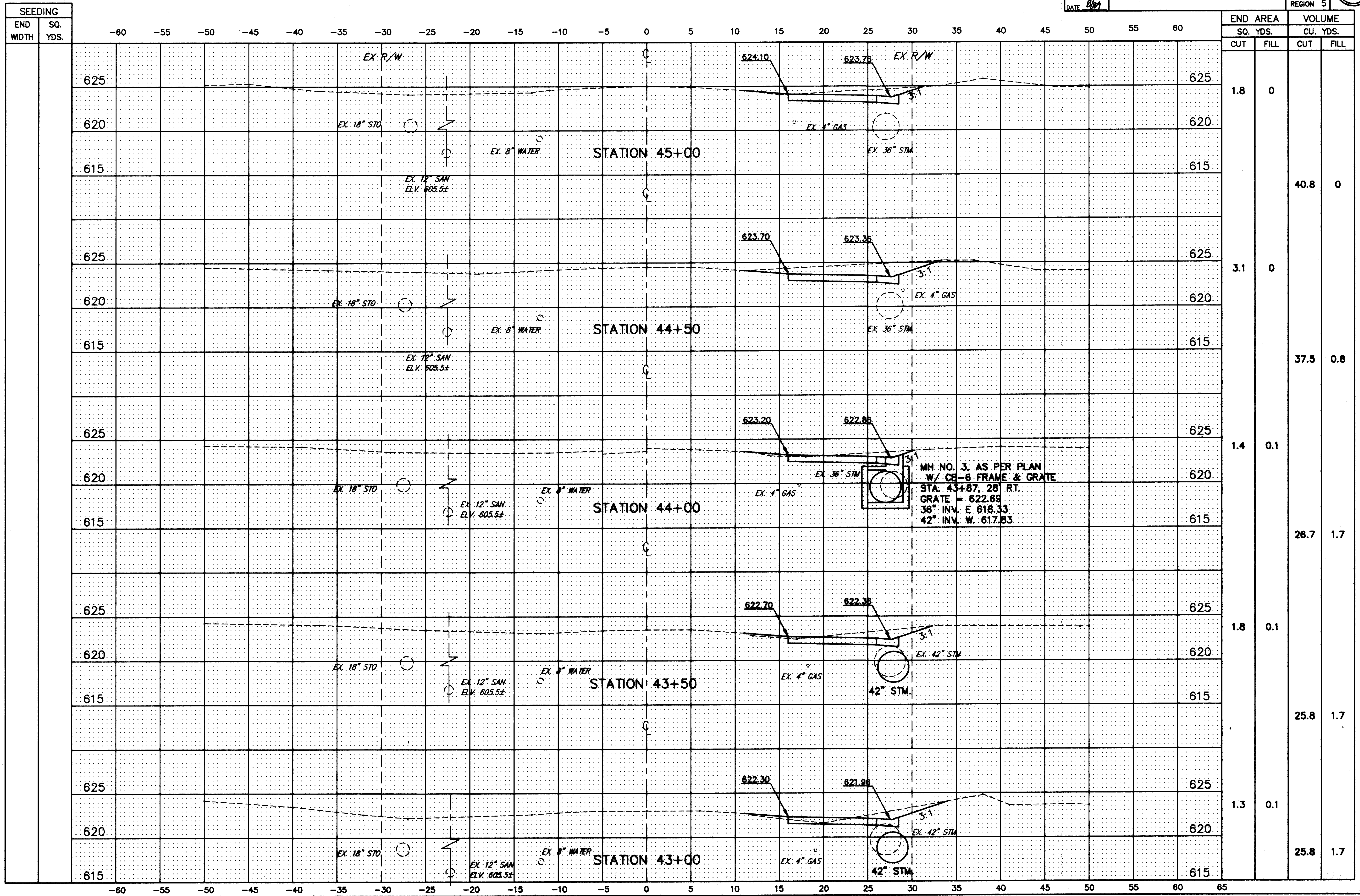
HENDRICKS ROAD CROSS-SECTIONS STA. 43+00 TO STA. 45+00
