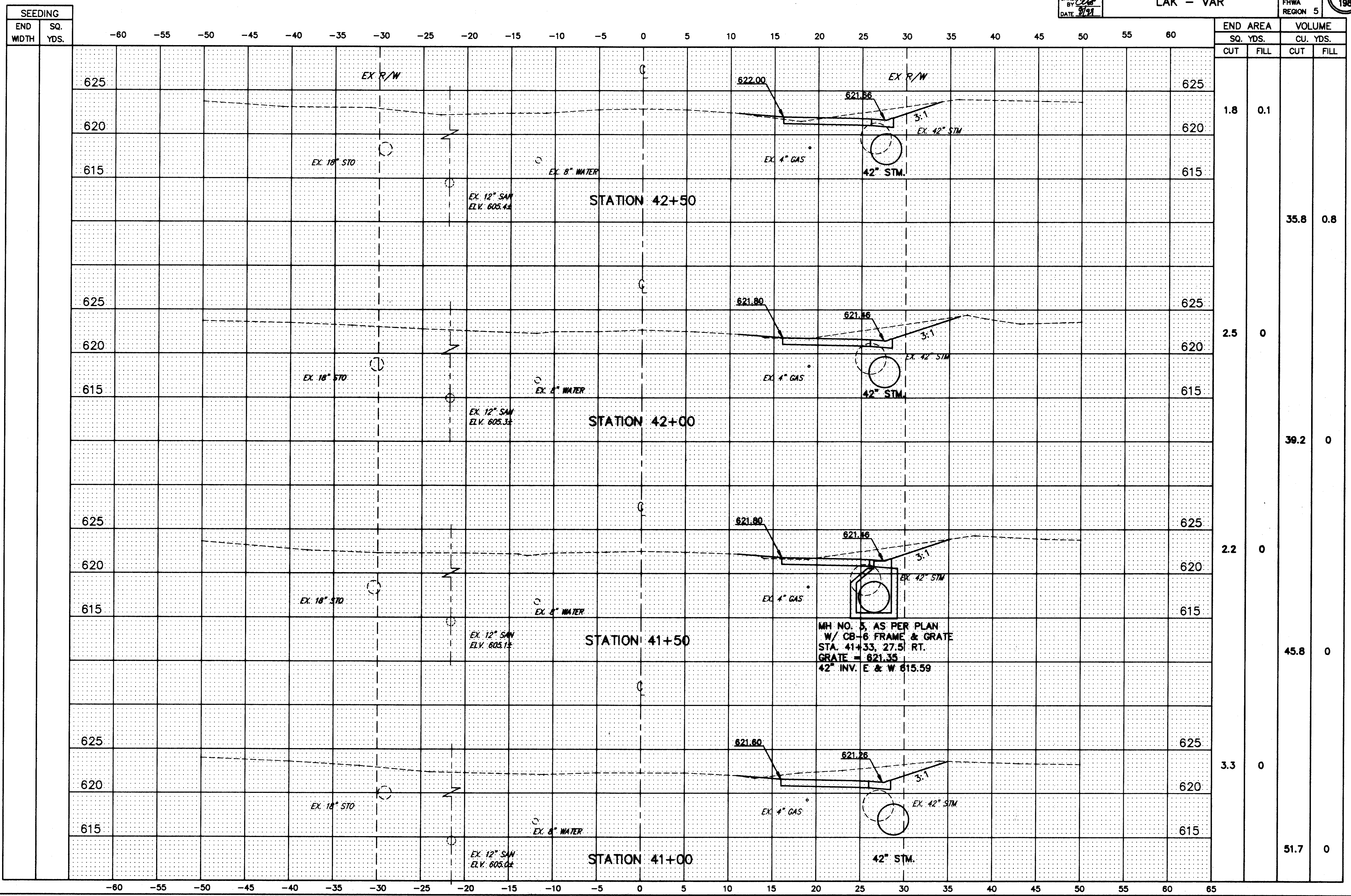
HENDRICKS ROAD CROSS-SECTIONS STA. 41+00 TO STA. 42+50
