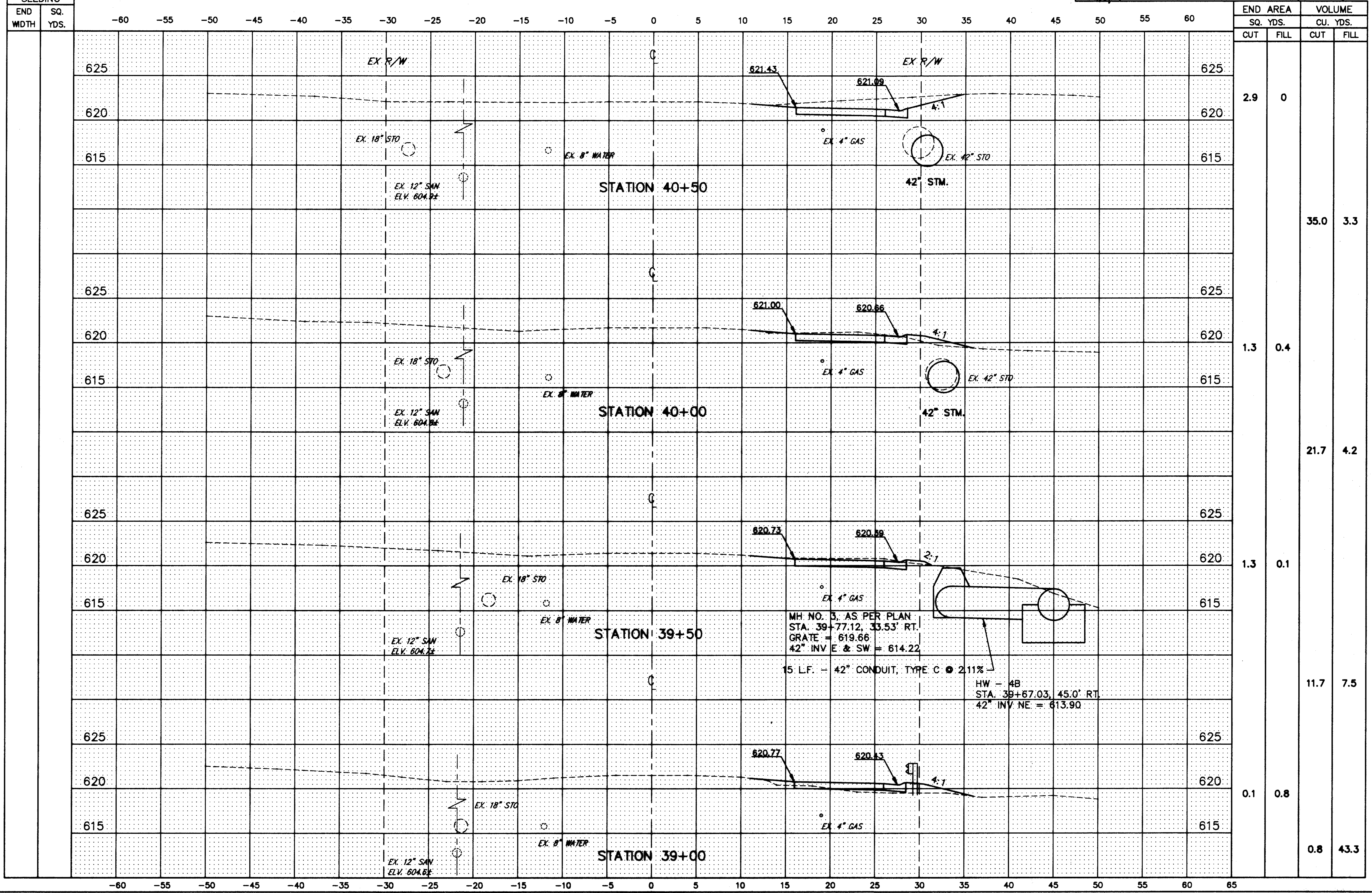
HENDRICKS ROAD CROSS-SECTIONS STA. 39+00 TO STA. 40+50
