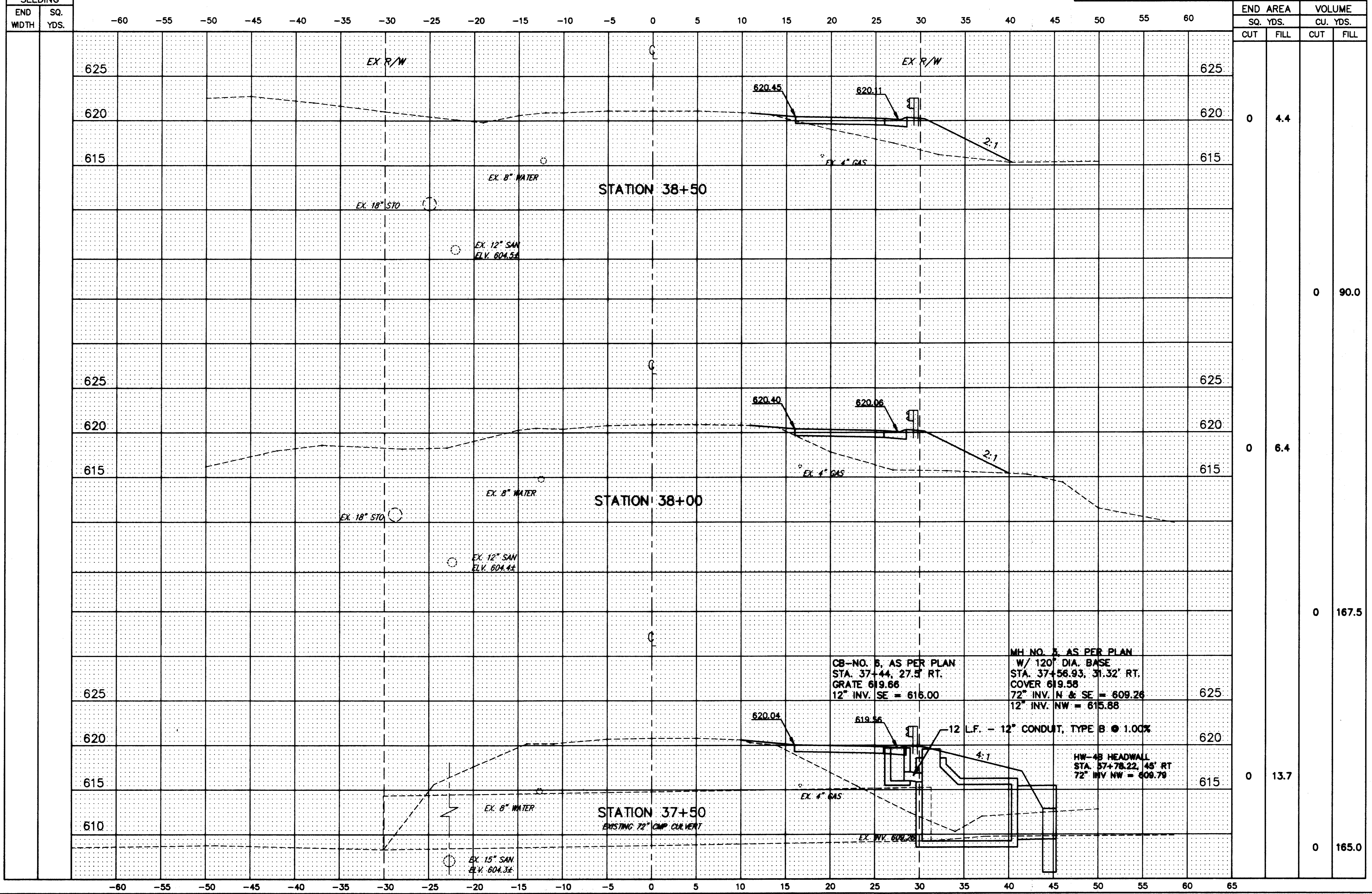
HENDRICKS ROAD CROSS-SECTIONS STA. 37+50 TO STA. 38+50
