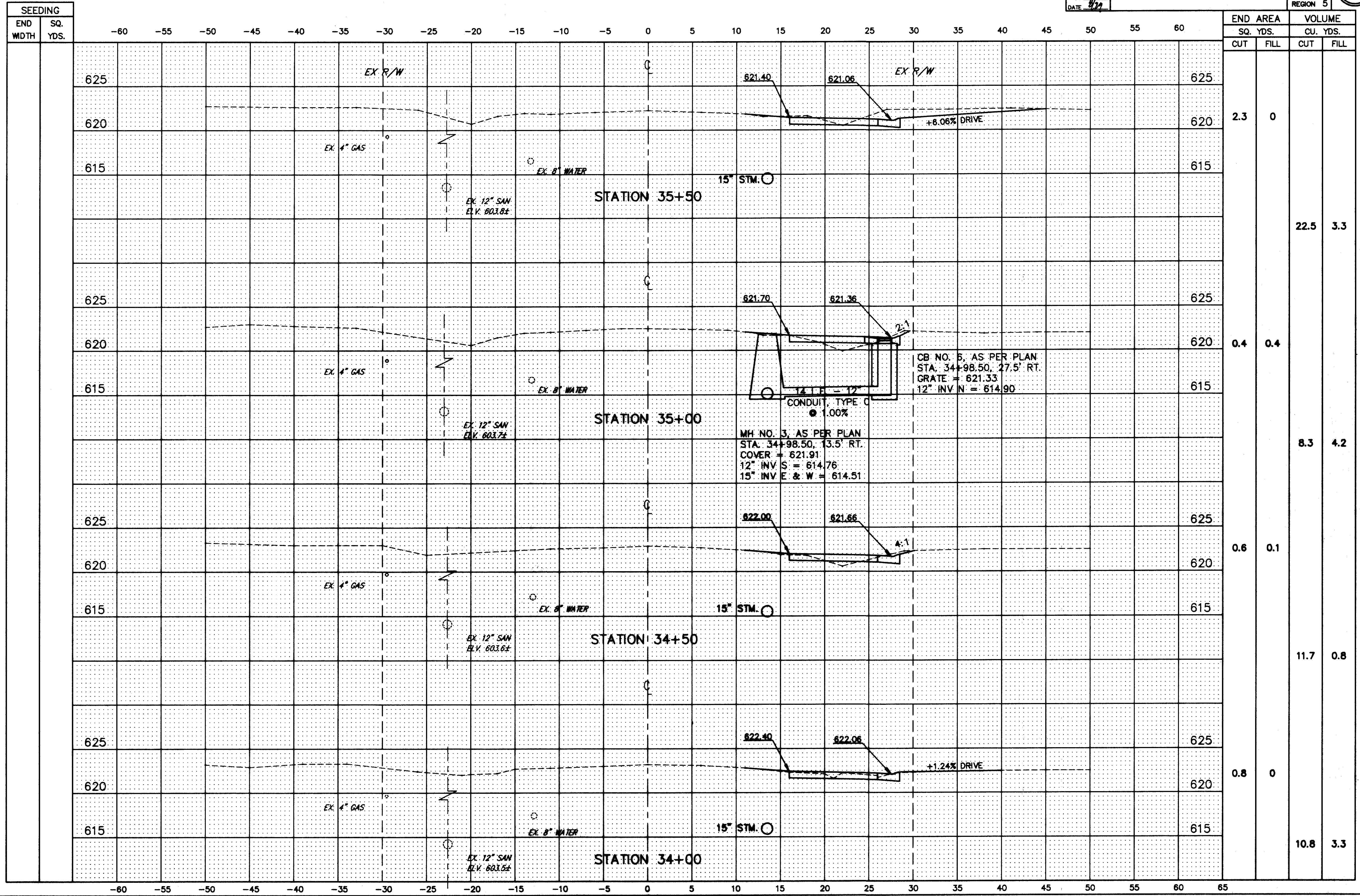
HENDRICKS ROAD CROSS-SECTIONS STA. 34+00 TO STA. 35+50
