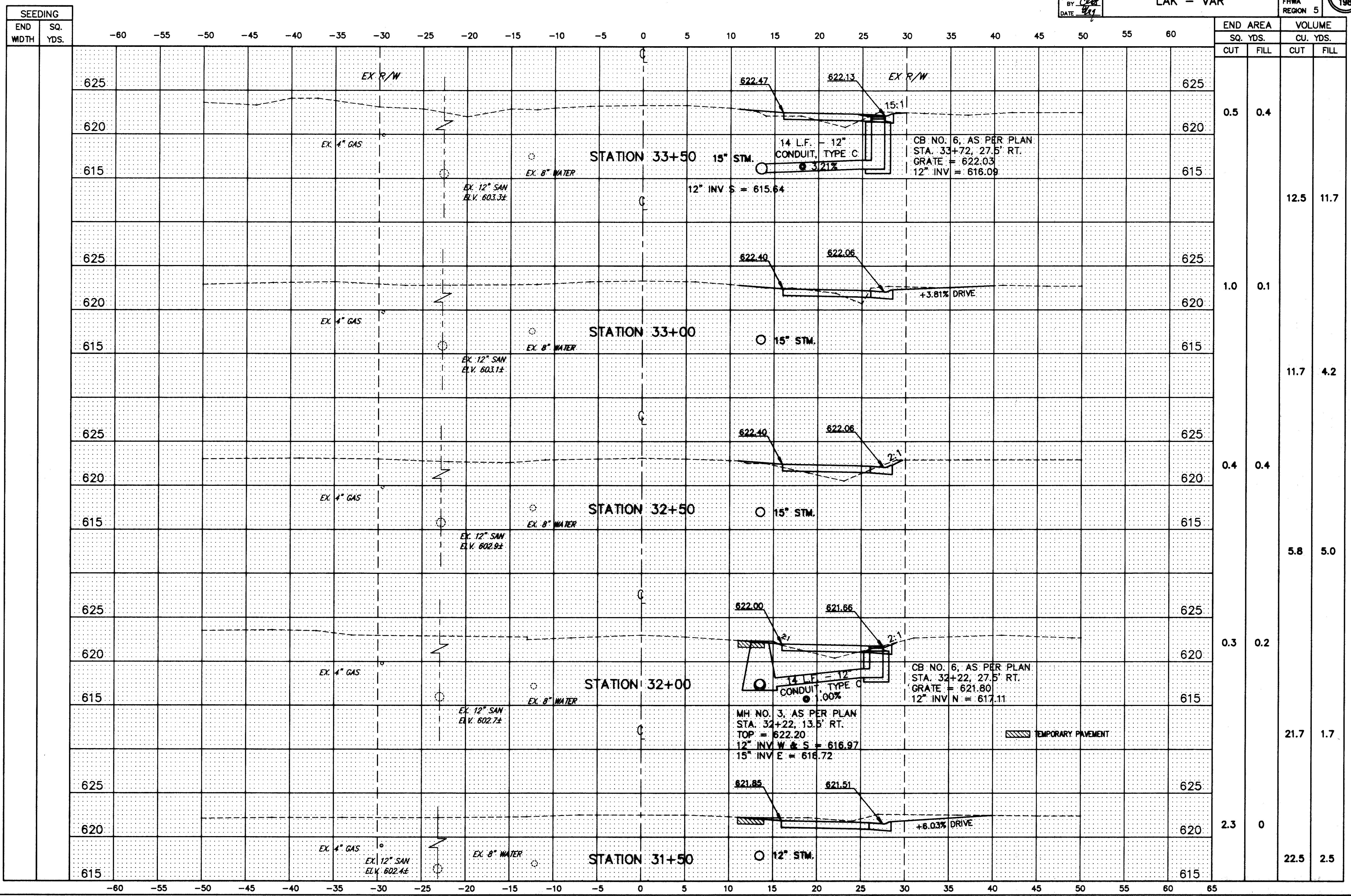
HENDRICKS ROAD CROSS-SECTIONS STA. 31+50 TO STA. 33+50
