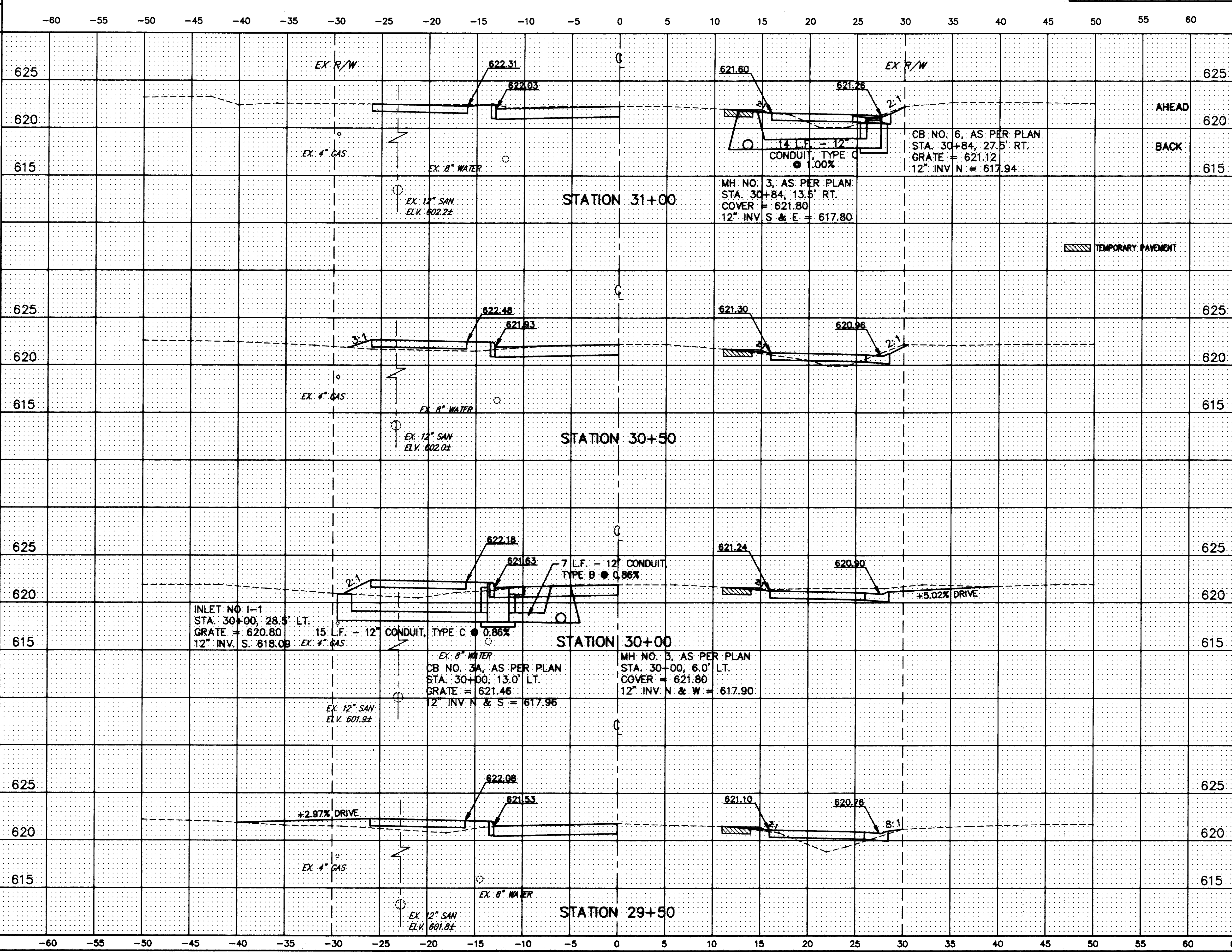
HENDRICKS ROAD CROSS-SECTIONS STA. 29+50 TO STA. 31+00
