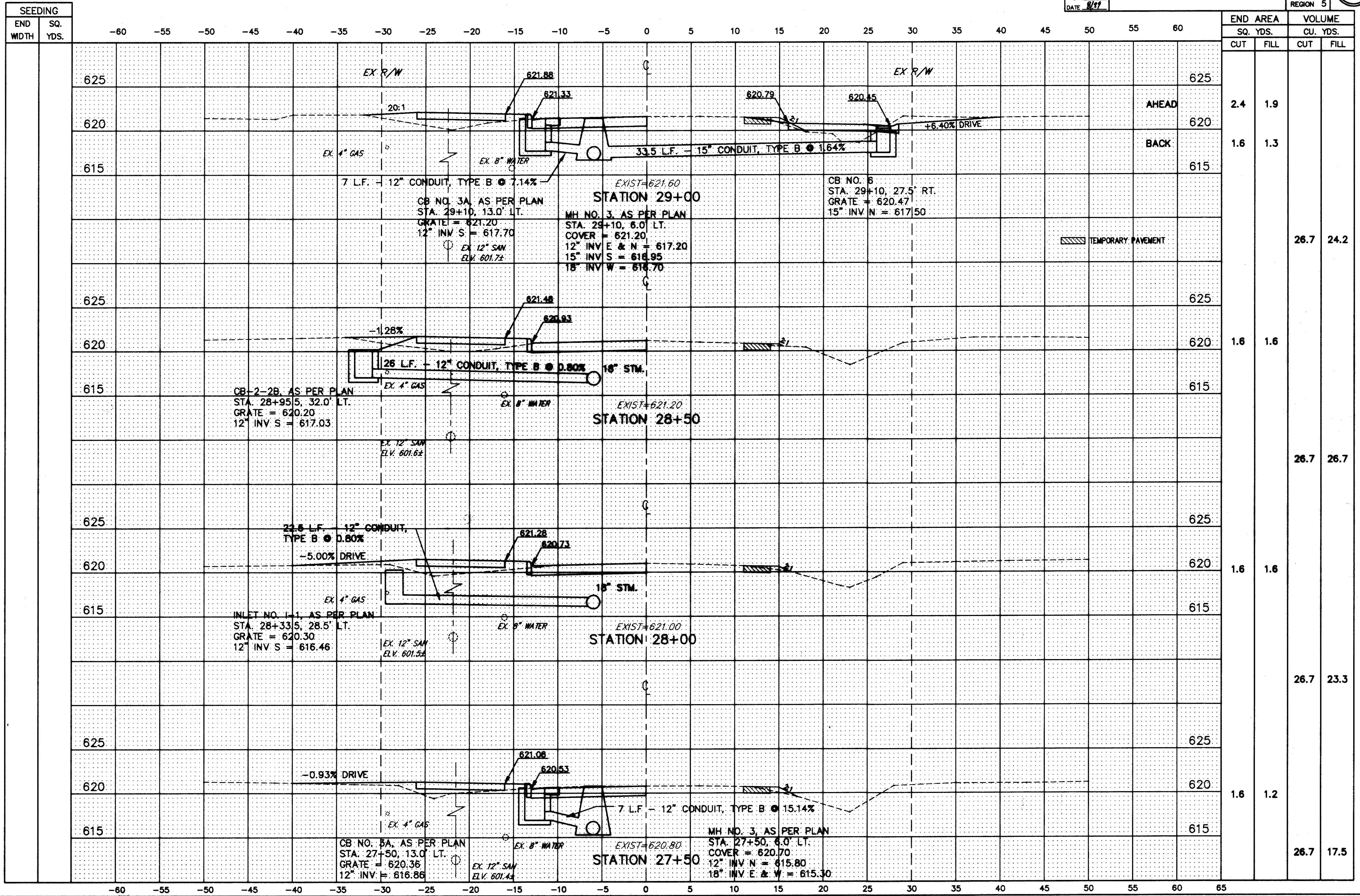
HENDRICKS ROAD CROSS-SECTIONS STA. 27+50 TO STA. 29+00
