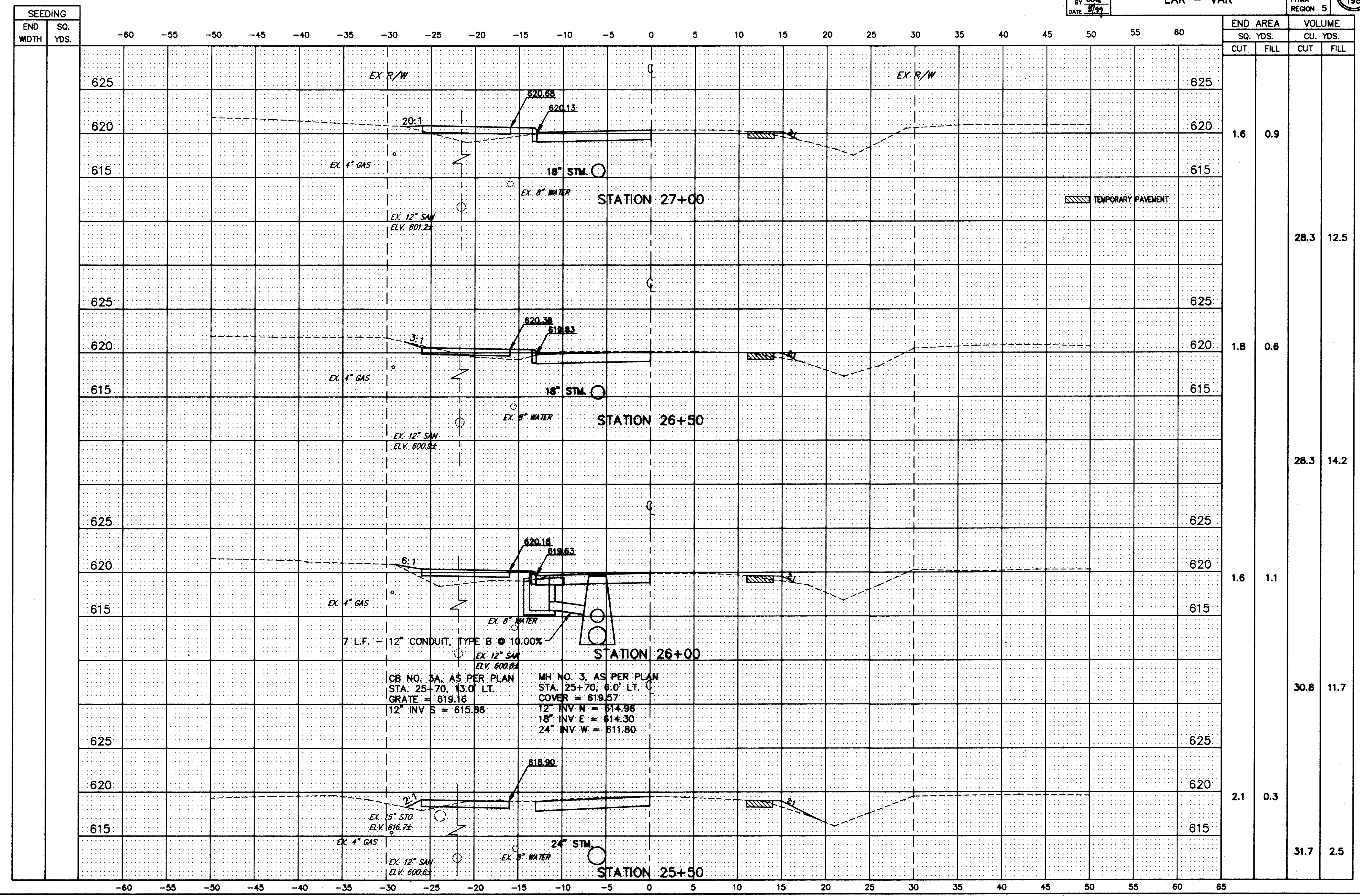
HENDRICKS ROAD CROSS-SECTIONS STA. 25+50 TO STA. 27+00
