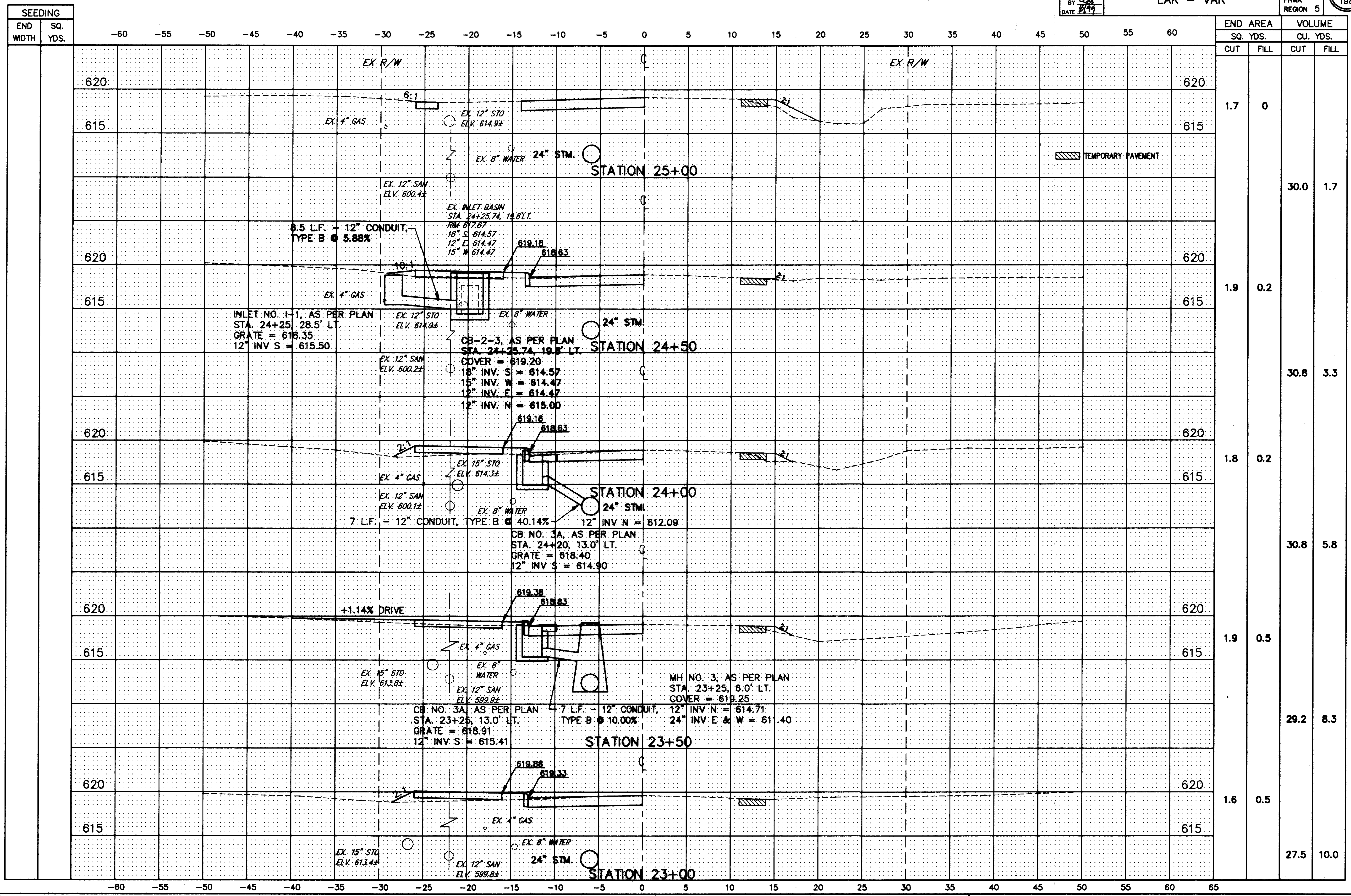
HENDRICKS ROAD CROSS-SECTIONS STA. 23+00 TO STA. 25+00
