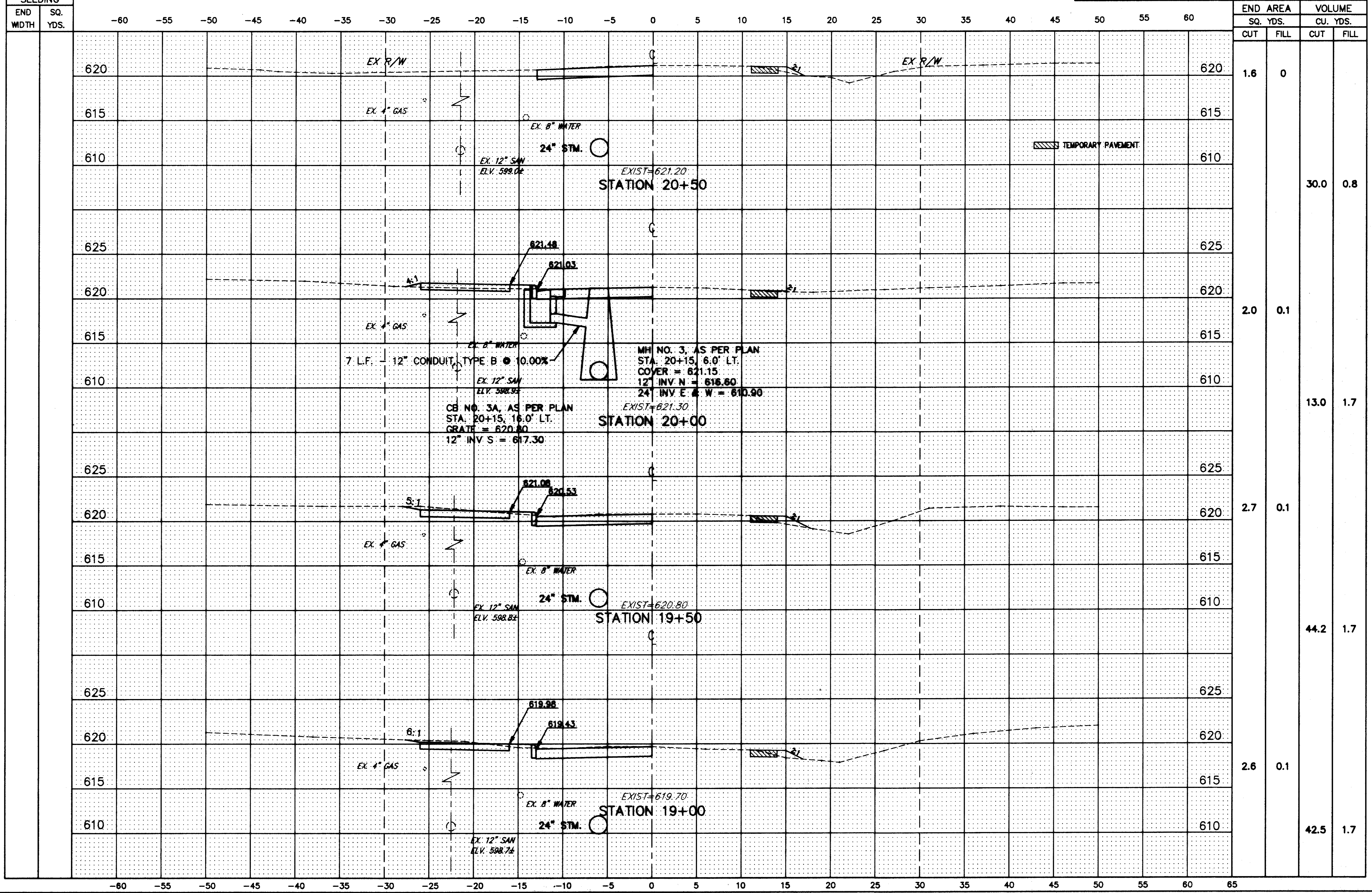
HENDRICKS ROAD CROSS-SECTIONS STA. 19+00 TO STA. 20+50
