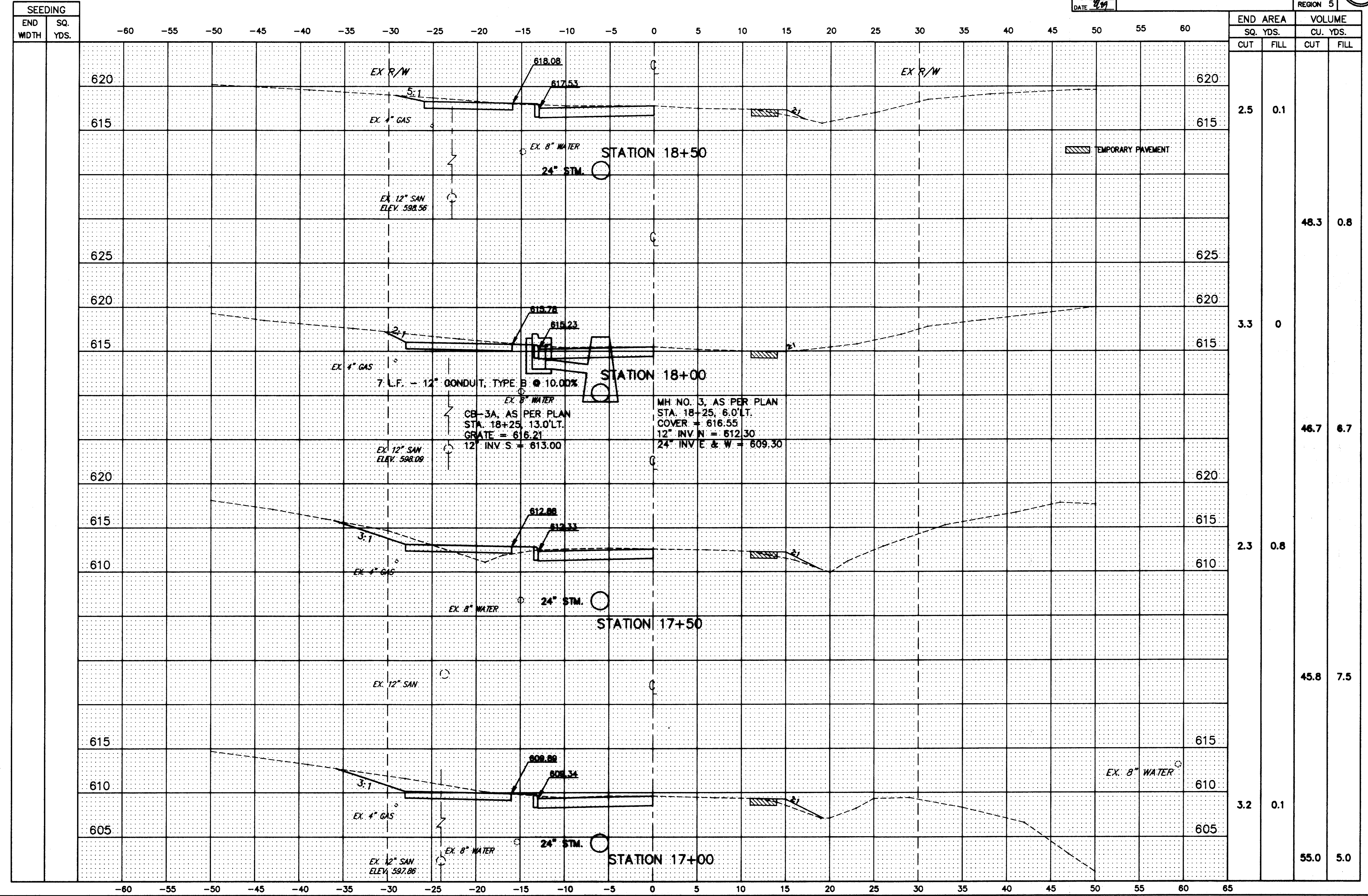
HENDRICKS ROAD CROSS-SECTIONS STA. 17+00 TO STA. 18+50
