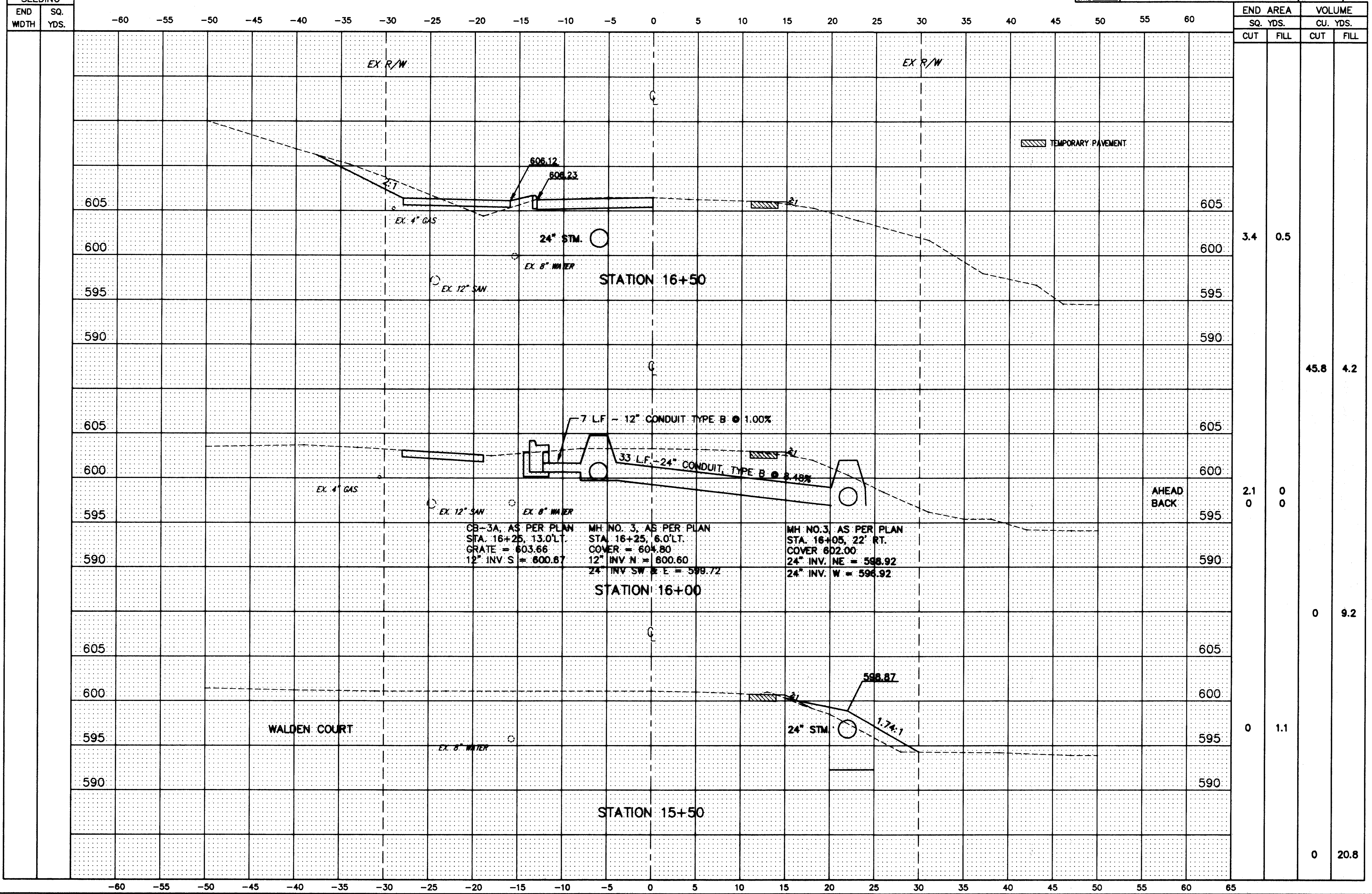
HENDRICKS ROAD CROSS-SECTIONS STA. 15+50 TO STA. 16+50
