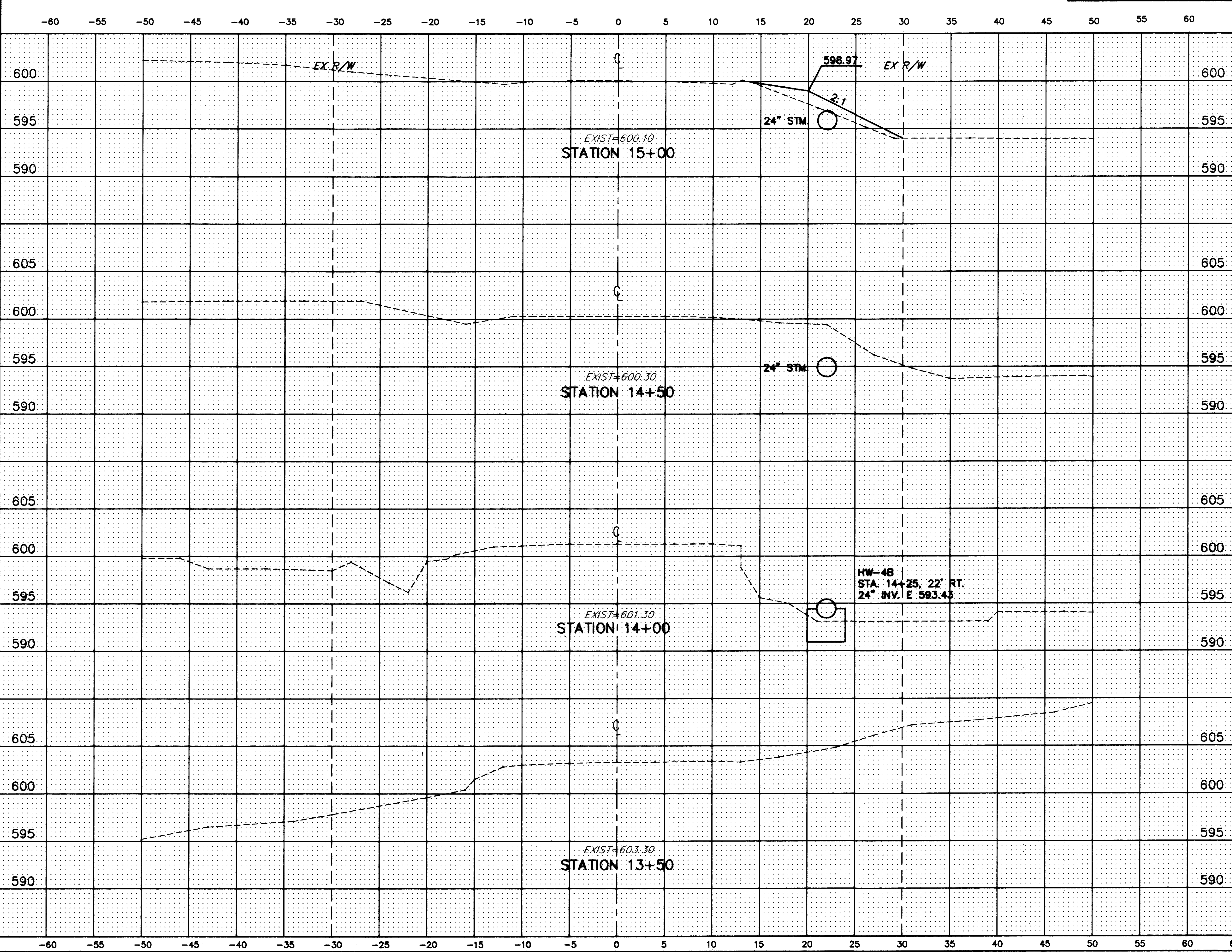
HENDRICKS ROAD CROSS-SECTIONS STA. 13+50 TO STA. 15+00
