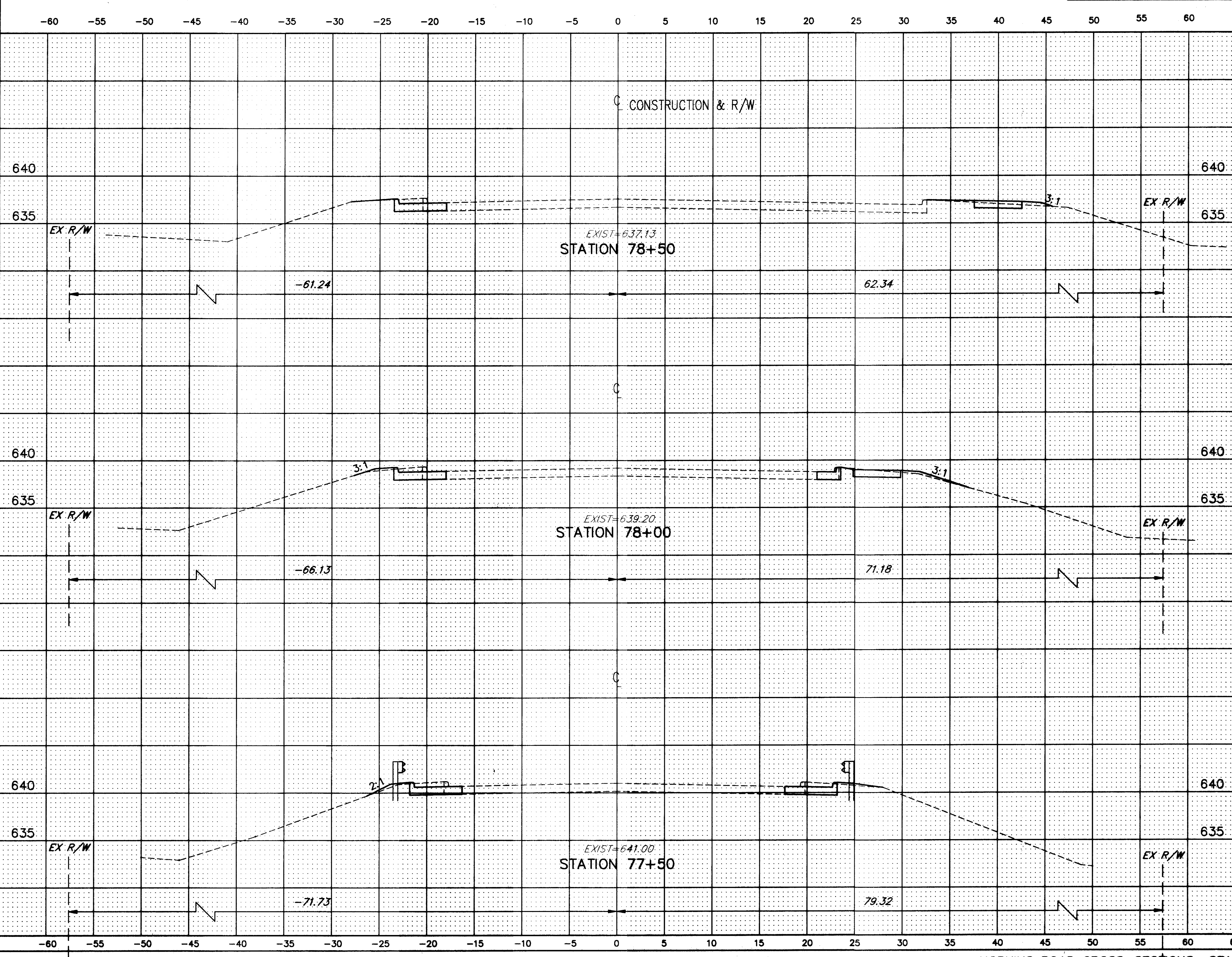
HOPKINS ROAD CROSS-SECTIONS STA. 77+50 TO STA. 78+50
